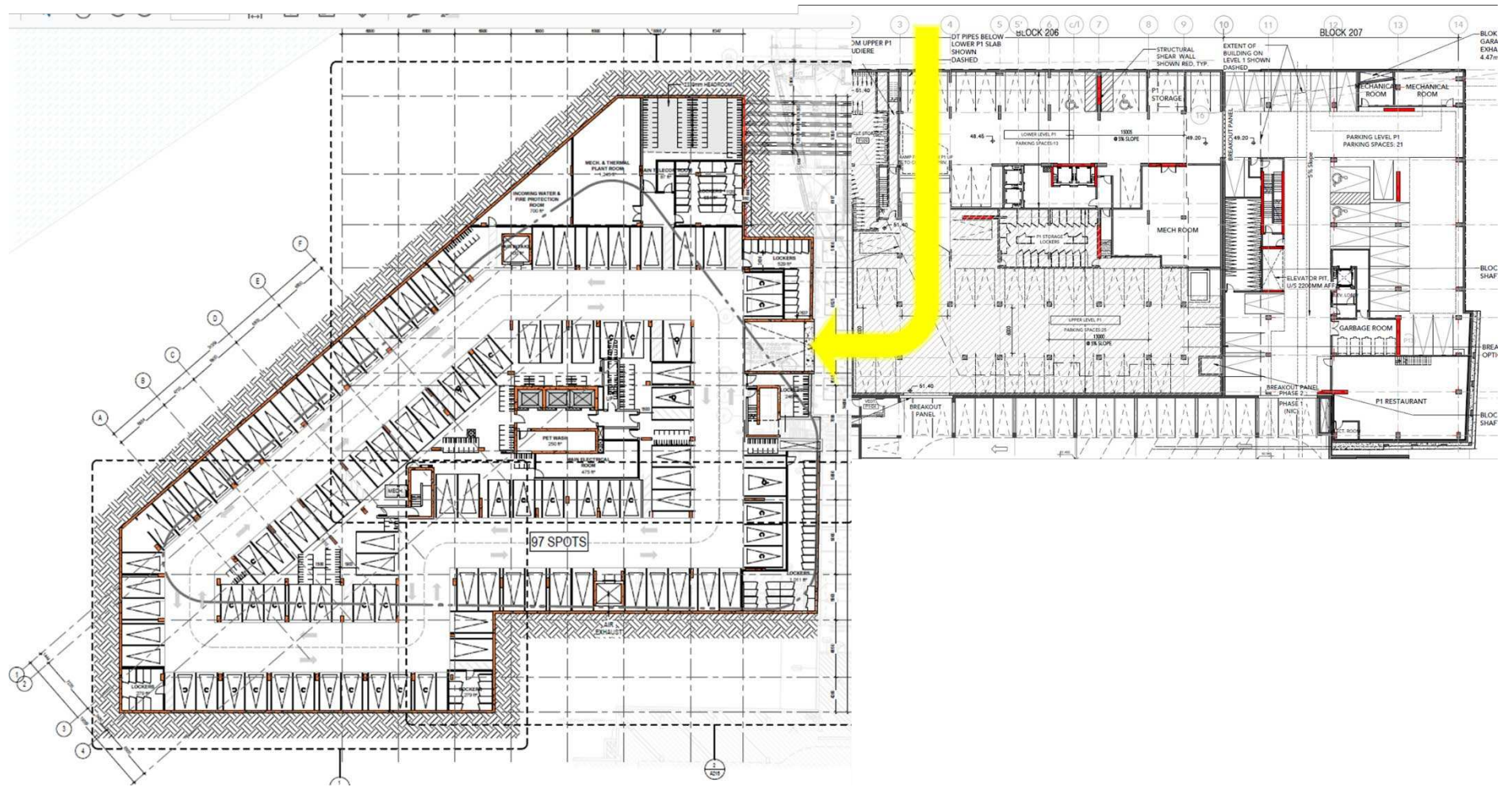
Figure 5: Block 204 On-site Vehicle Circulation (underground parking)
