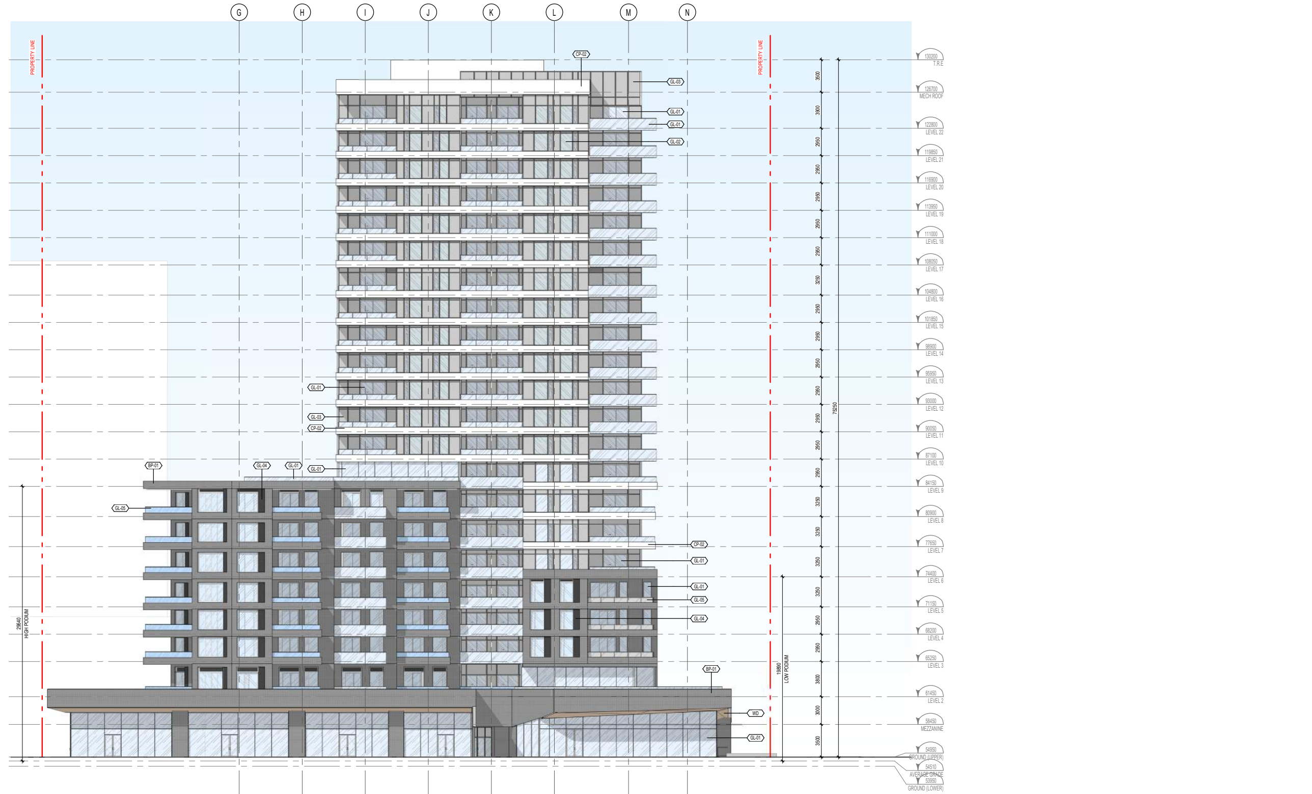
SOUTH ELEVATION
