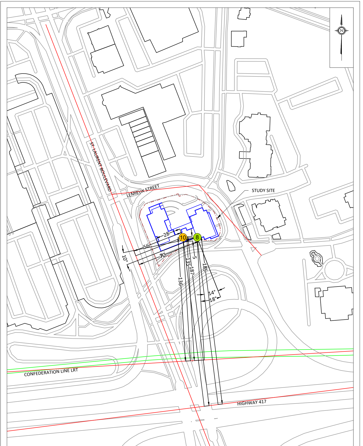
FIGURE 8: STAMSON INPUT PARAMETERS - RECEPTOR 8,10
