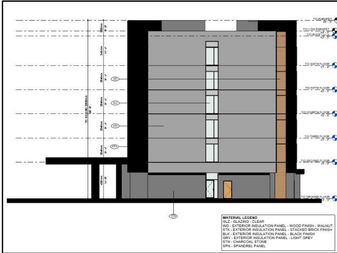
South Elevation
