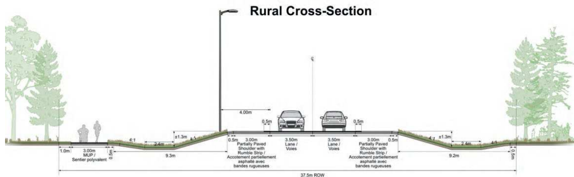
Figure 5 - Earl Armstrong Road Extension Cross-Section: Bank Street to Hawthorne Road
