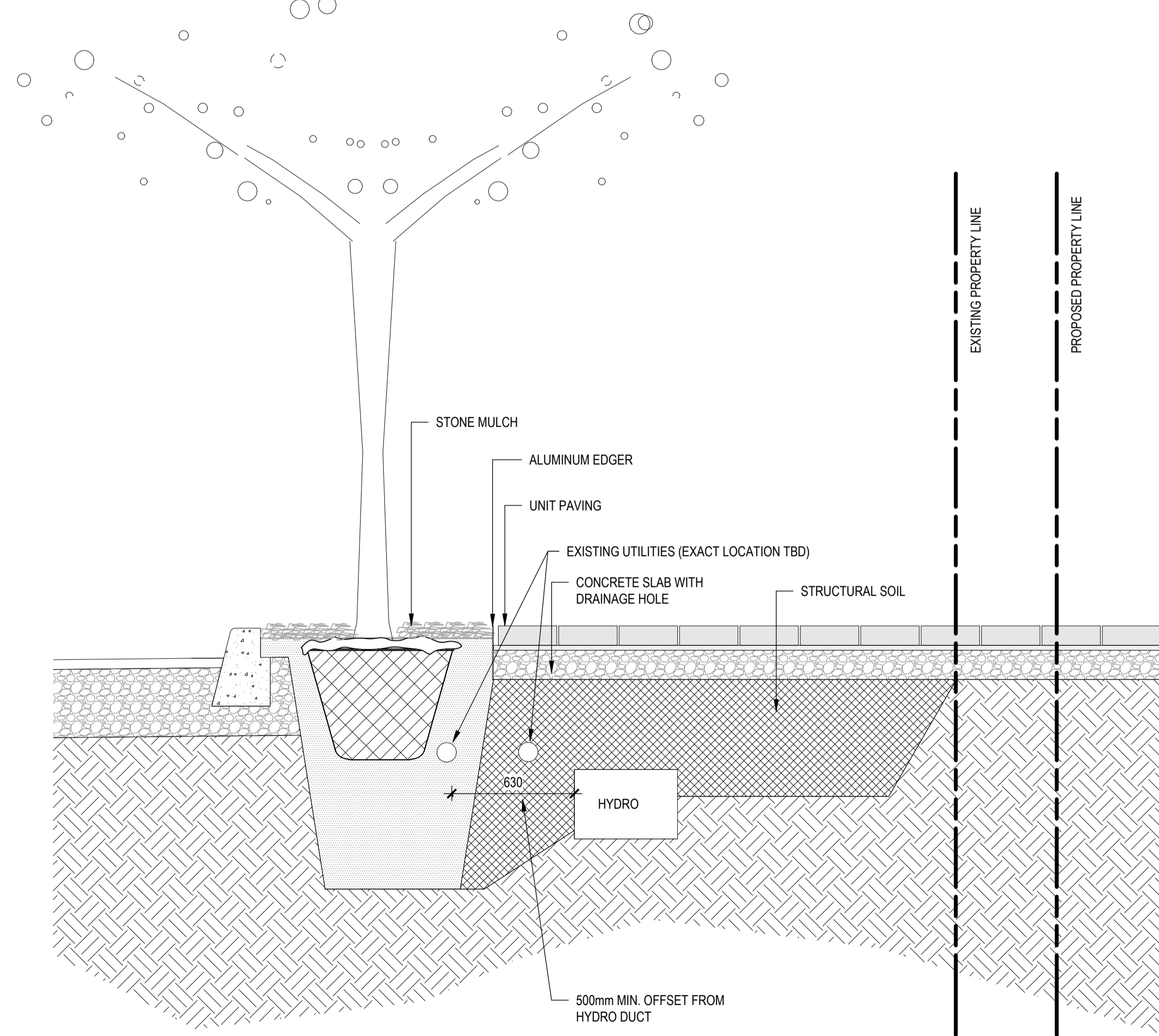
3 SECTION THROUGH WELLINGTON STREET TREE SCALE: 1:20
