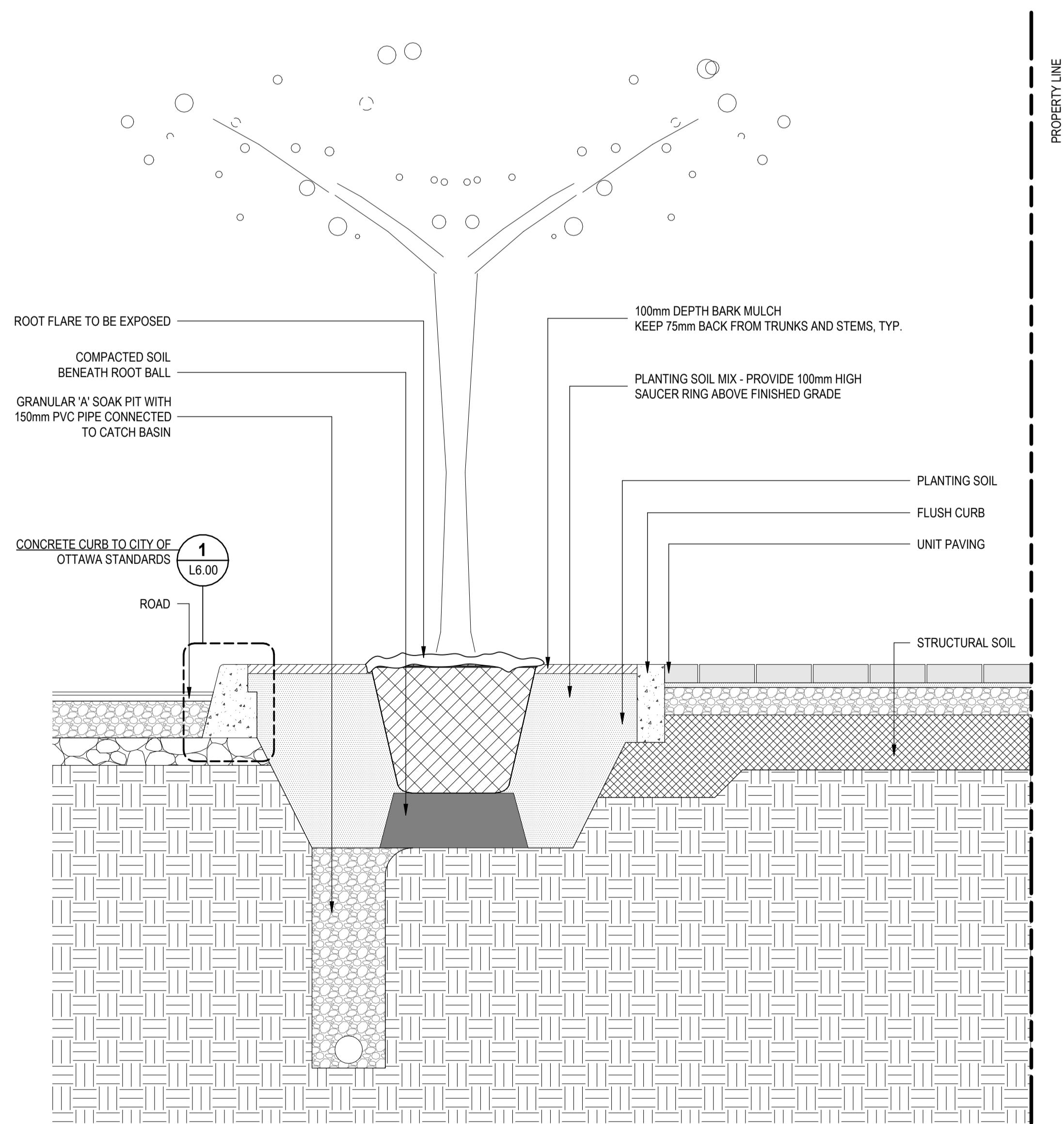
2 SECTION THROUGH OPEN PLANTER SCALE: 1:20
