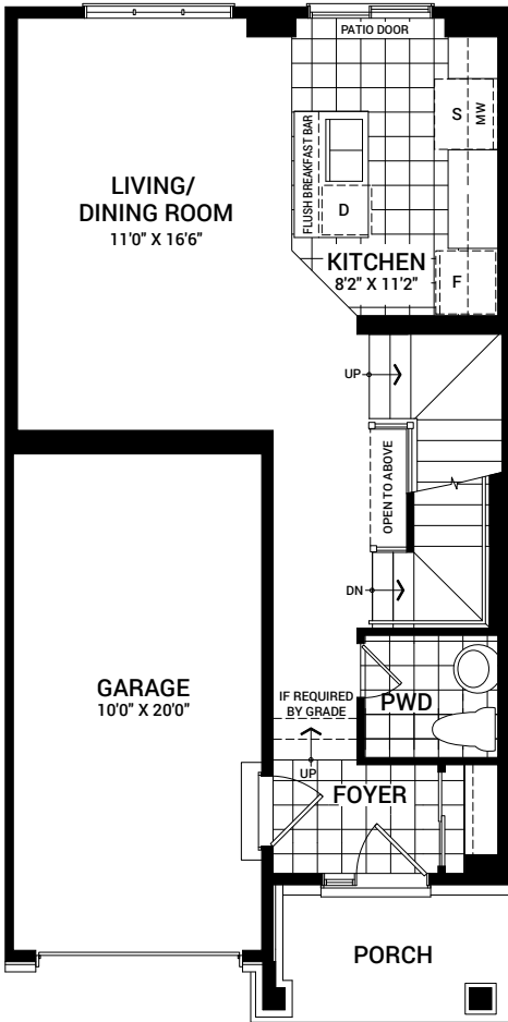
MAIN FLOOR PLAN B
