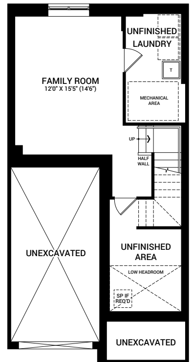
BASEMENT FLOOR PLAN
