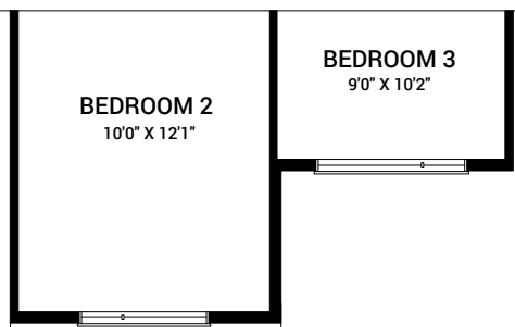
SECOND FLOOR PLAN D
