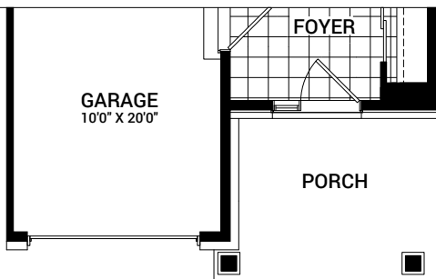
MAIN FLOOR PLAN C
