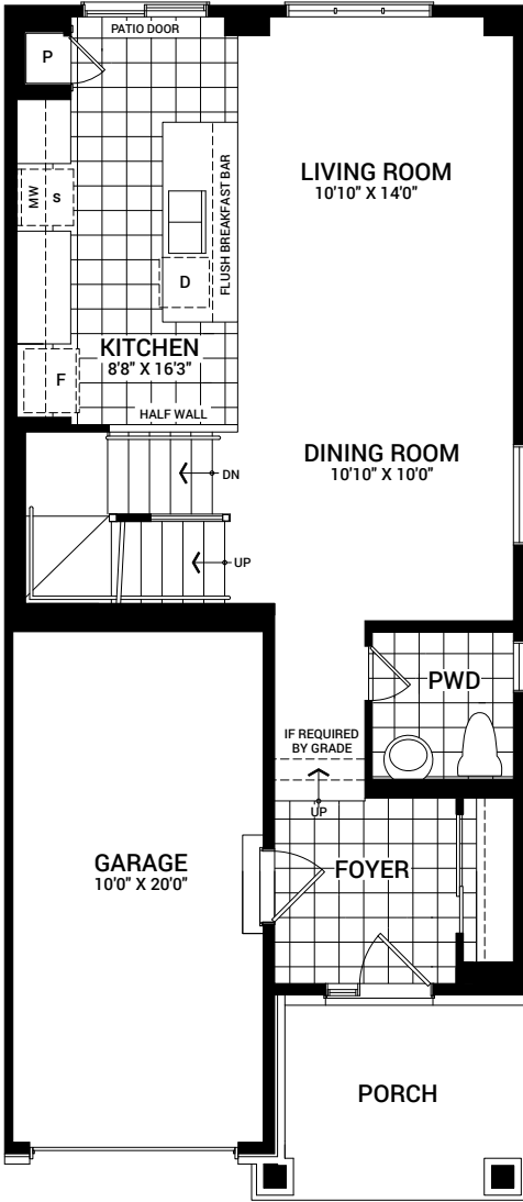
MAIN FLOOR PLAN B
