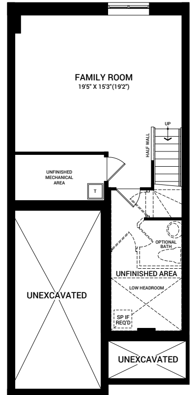
BASEMENT PLAN
