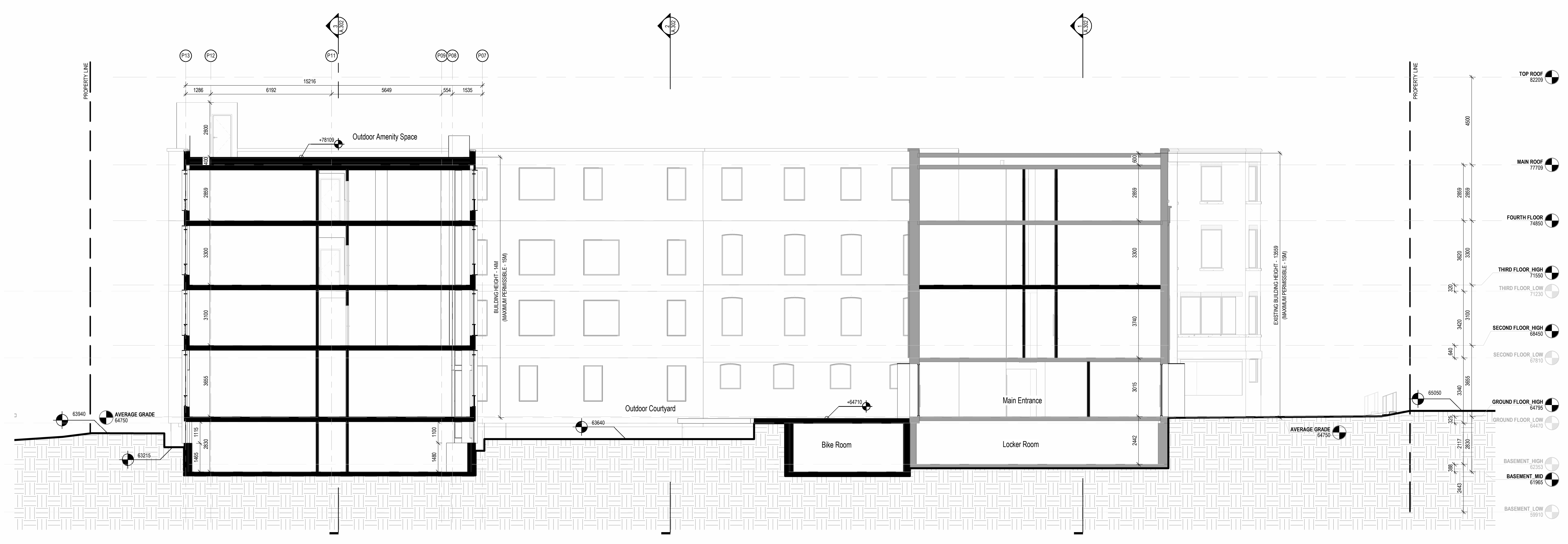
SECTION - NS II 1:100
