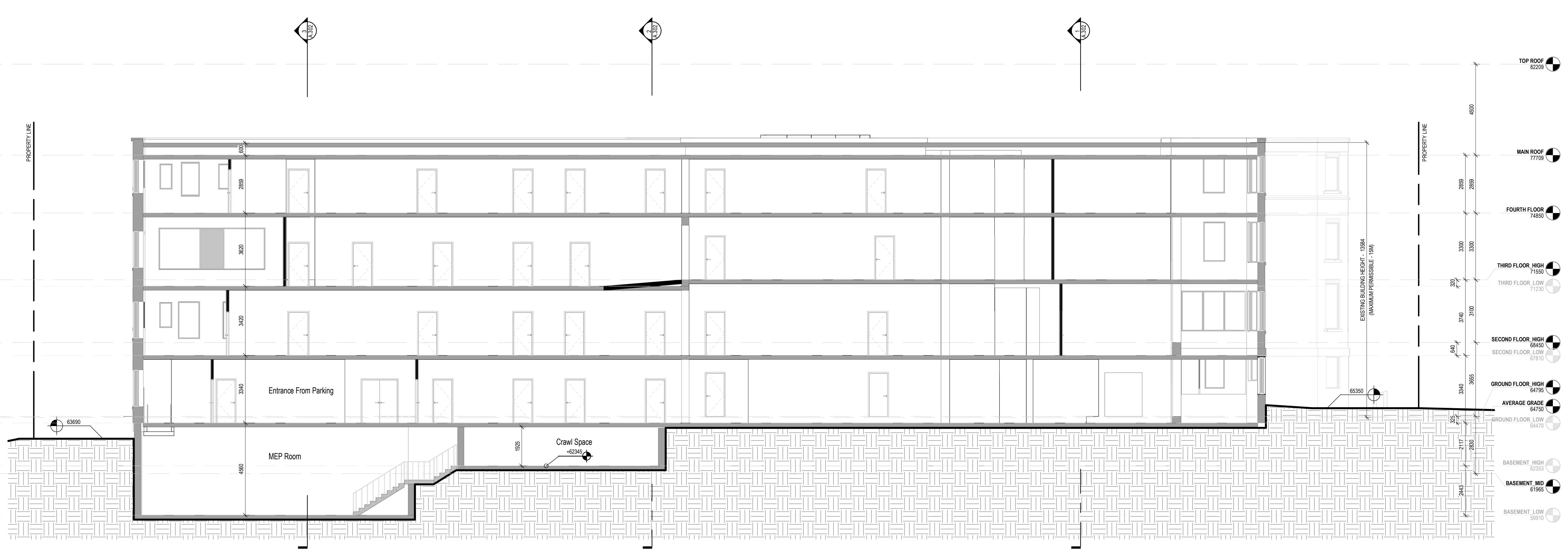
SECTION - NS III 1:100
