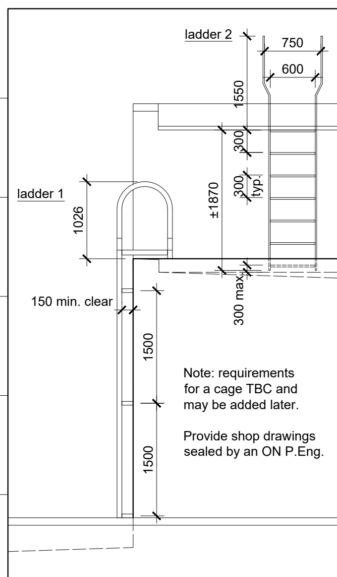
roof ladders, south elev. ELEVATION 2 : 50
