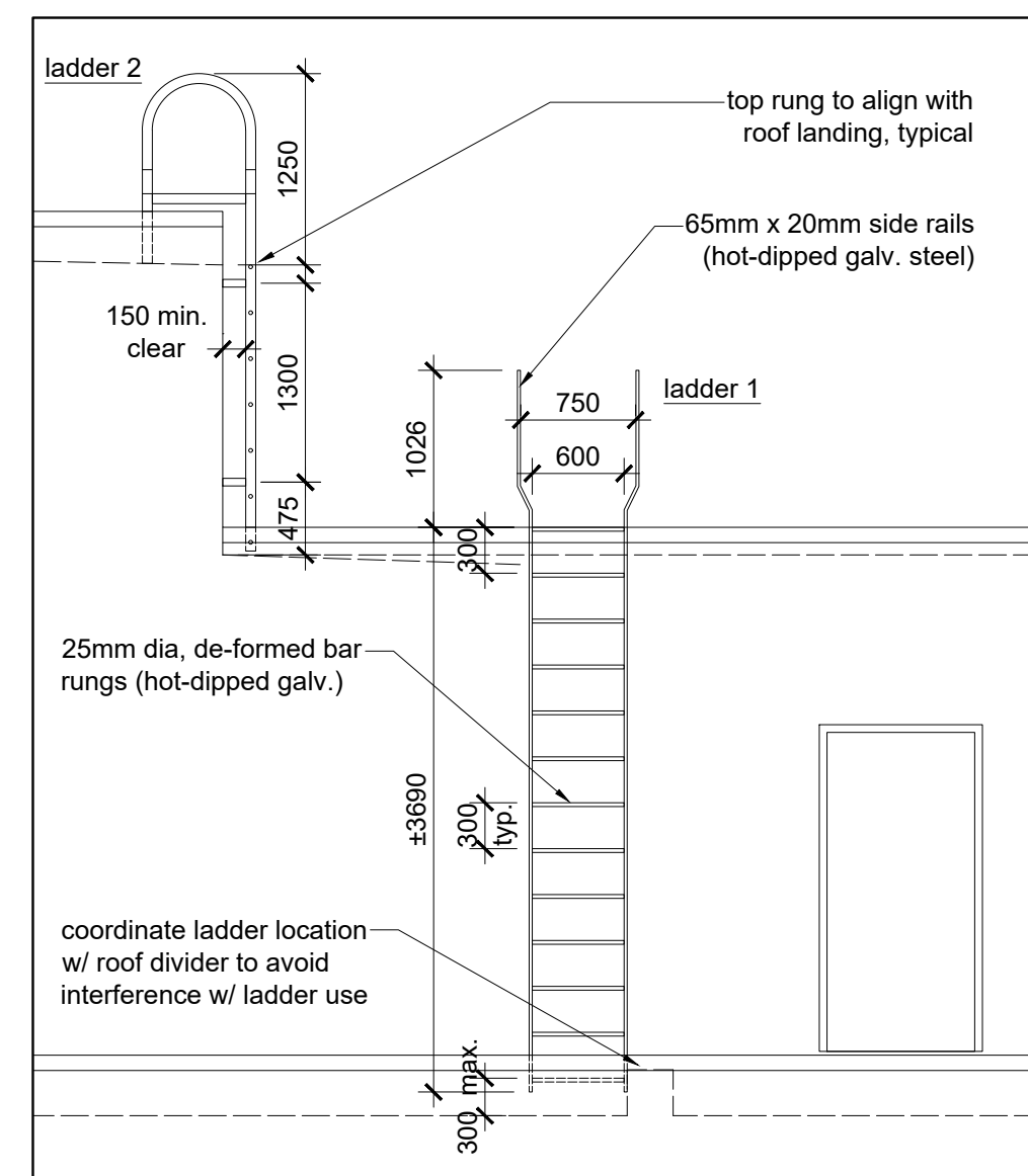
roof ladders, west elev. ELEVATION 2 : 50
