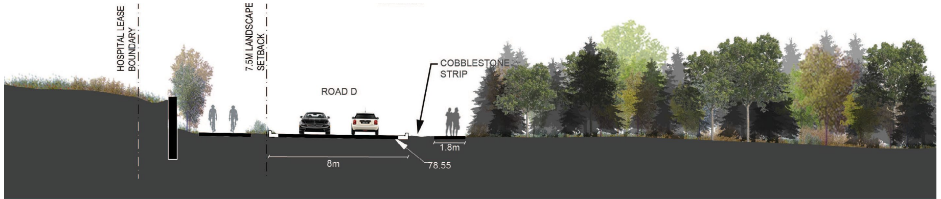
Figure 53: Section D Looking north at South Property Line.
