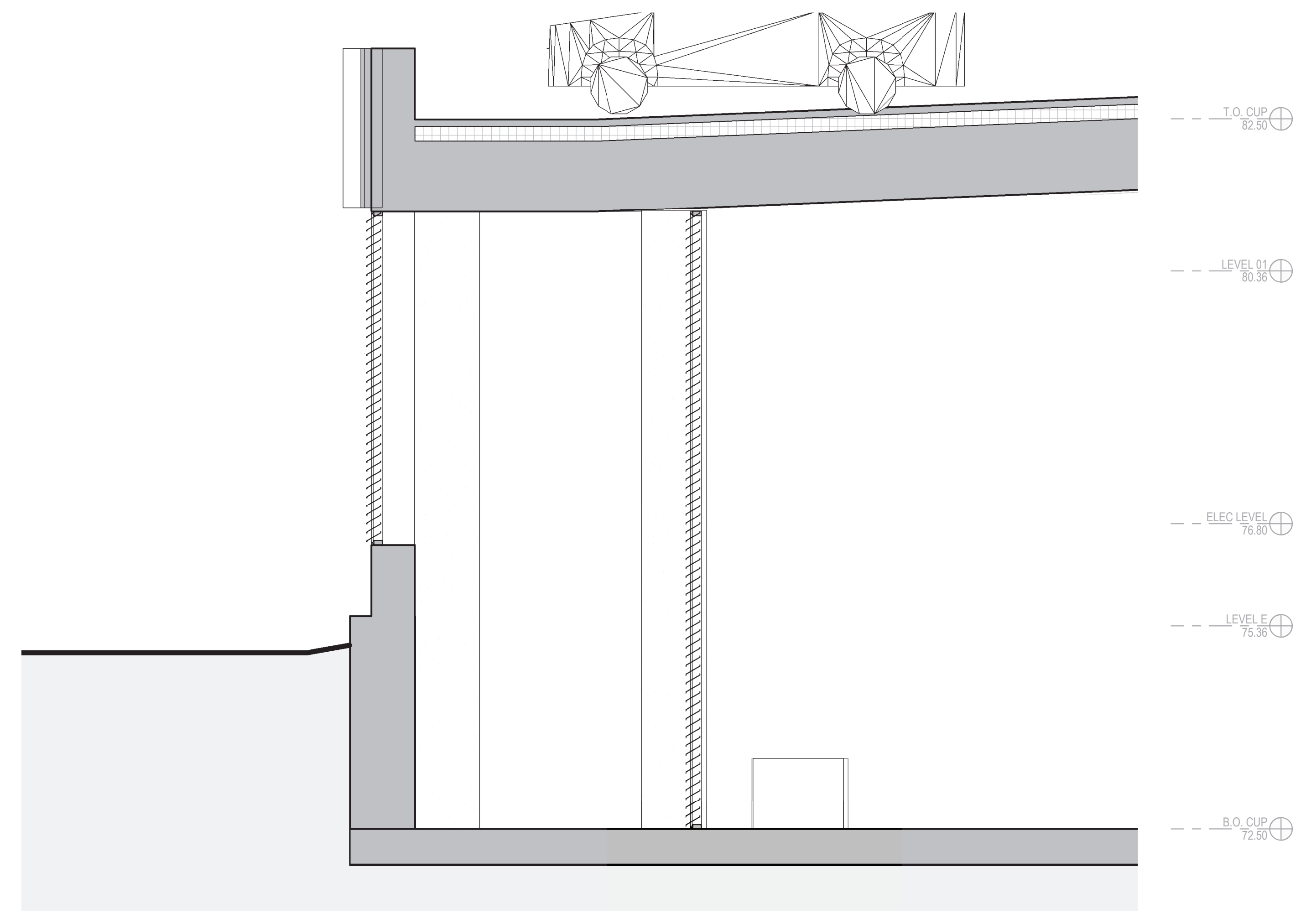
1 SECTION 1:50
