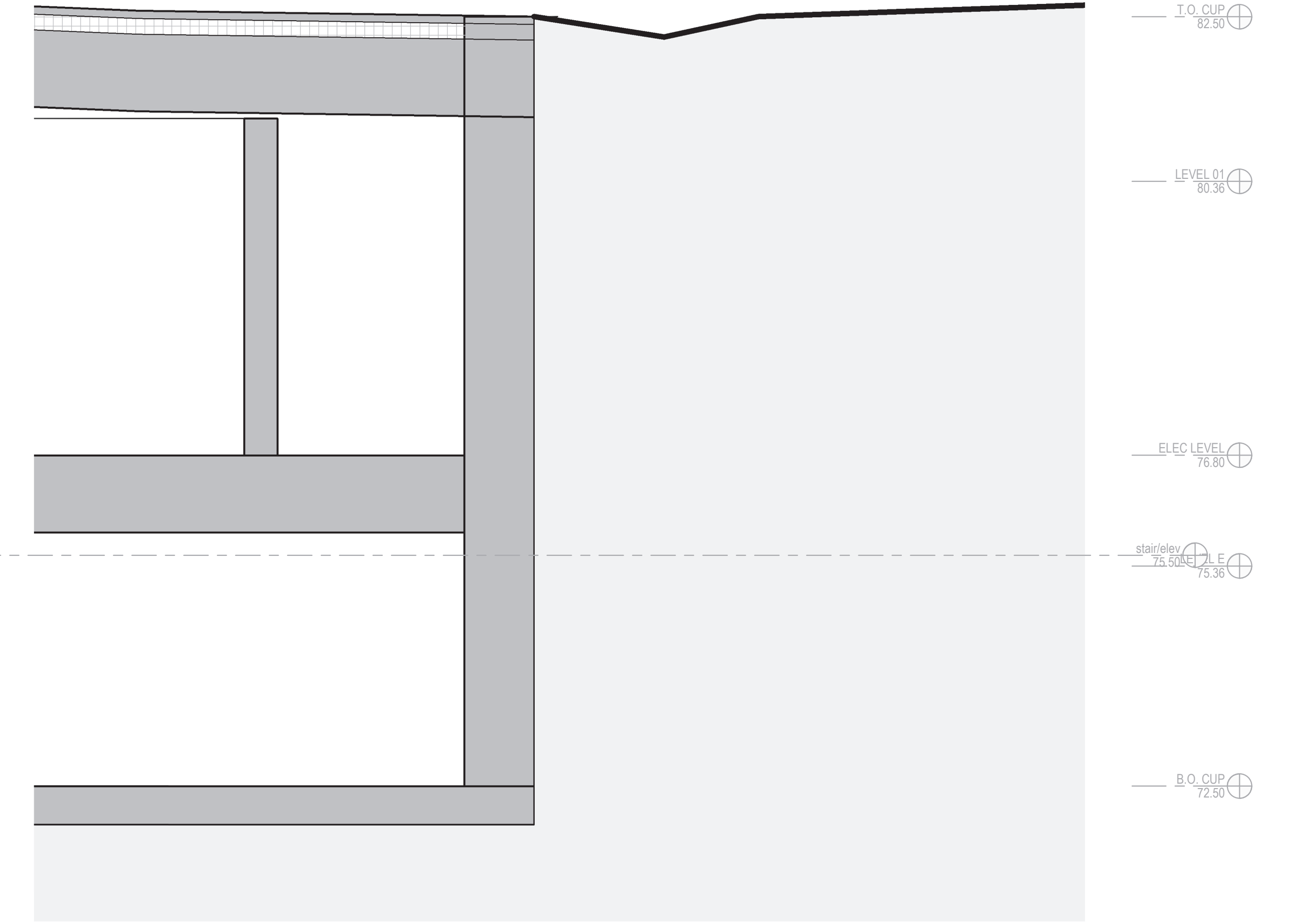
3 SECTION 1:50
