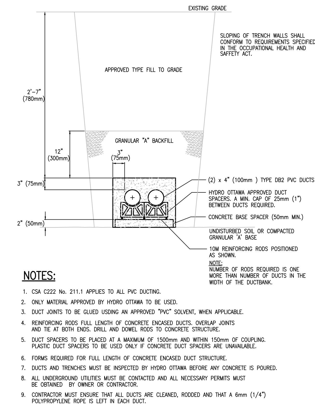
3 E2 2-CELL CONCRETE DUCT BANK FOR SECONDARY SERVICE N.T.S.
