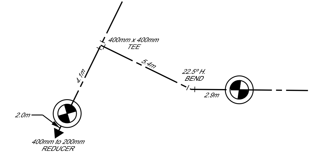
400mm WATERMAIN DETAIL @ STA. 6+025.799
