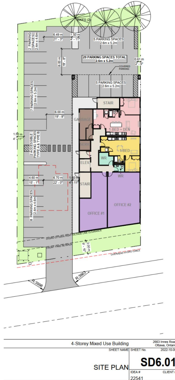
Figure 1.1 – Site plan of 2663 Innes Road.
