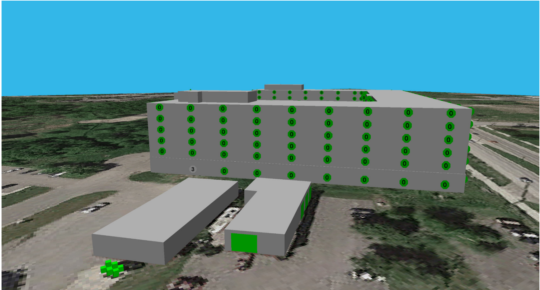
Figure 6b: Stationary Noise Excesses at Southwest Façade, Evening, Leq [dBA]
