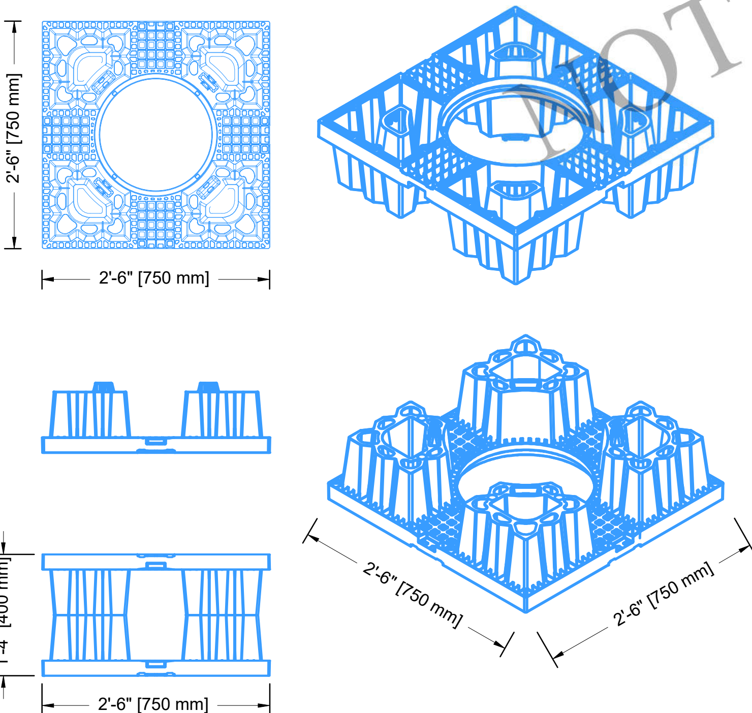
2 AQUABOX CUBE HP S-03
