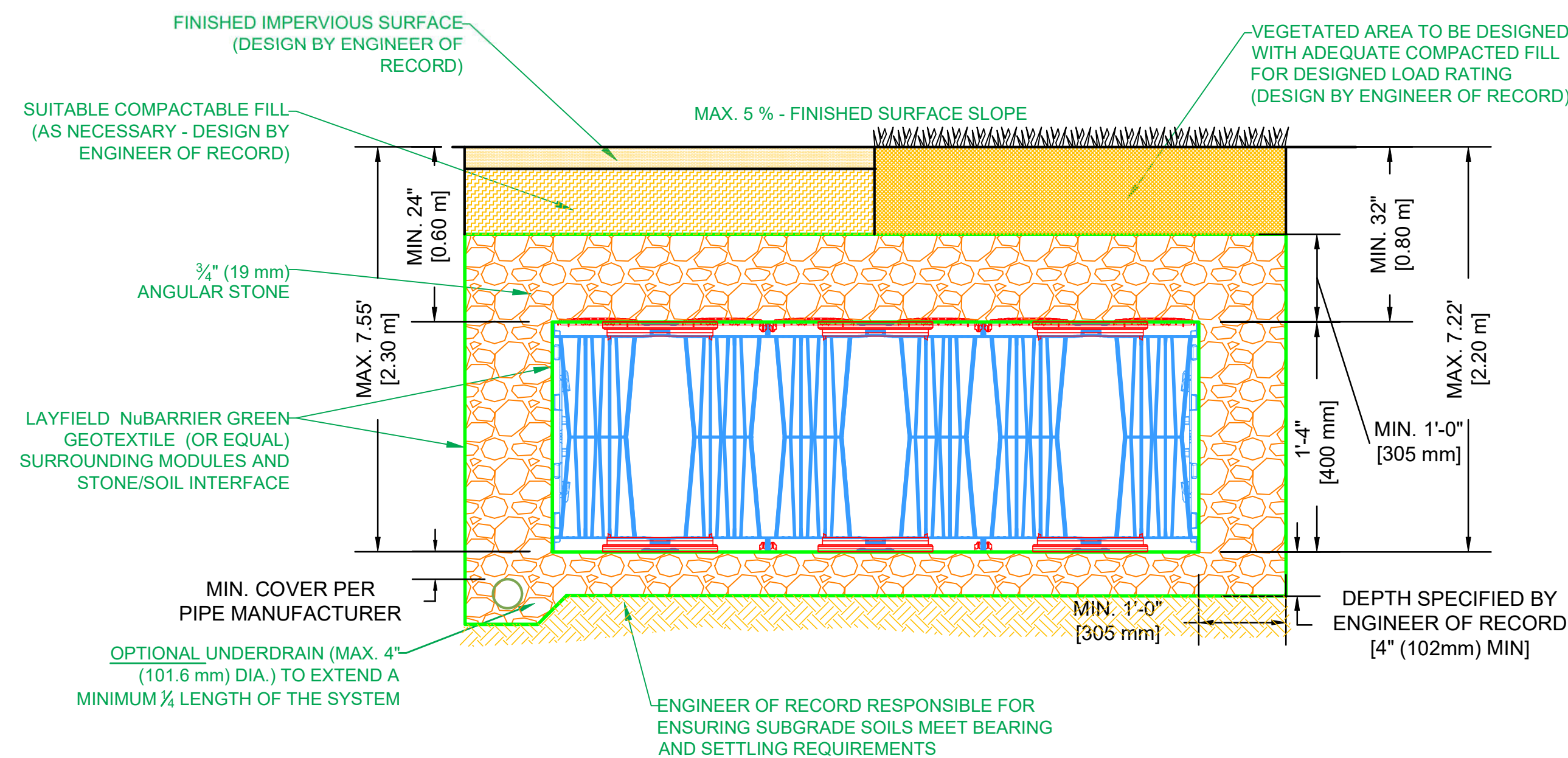
5 TYPICAL SYSTEM CROSS SECTION S-03
