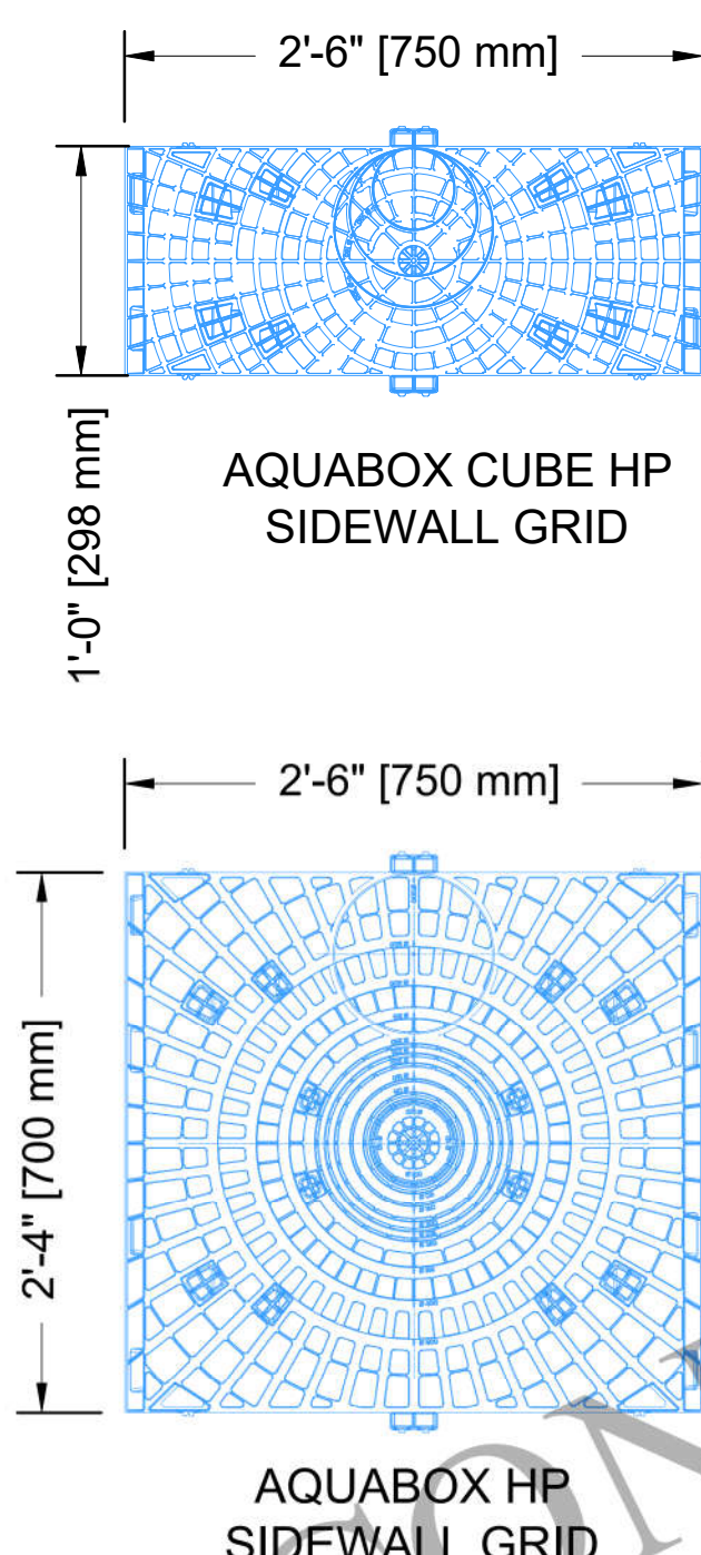
3 AQUABOX SIDEWALL GRID S-03
