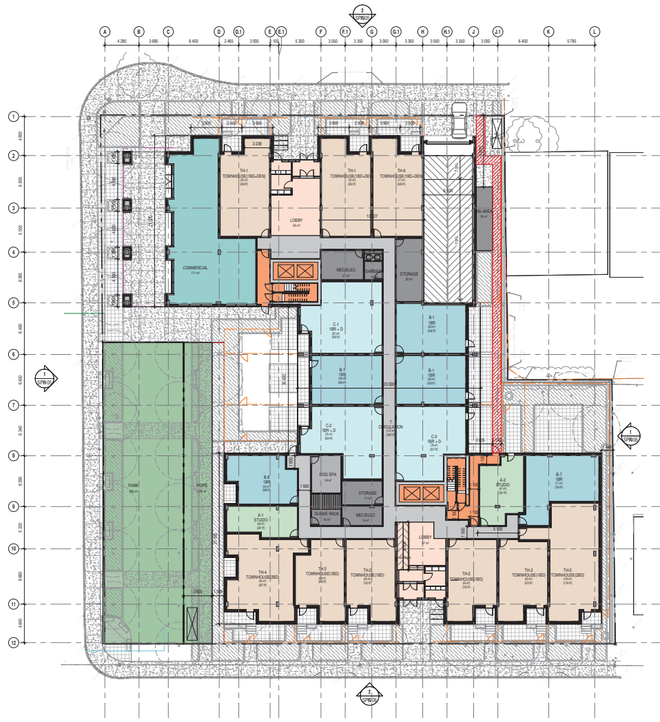
GROUND FLOOR 1:200
