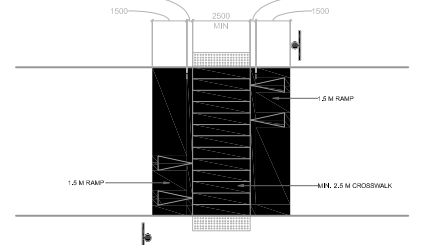
RAISED CROSSWALK - TYPICAL PLAN DETAIL
