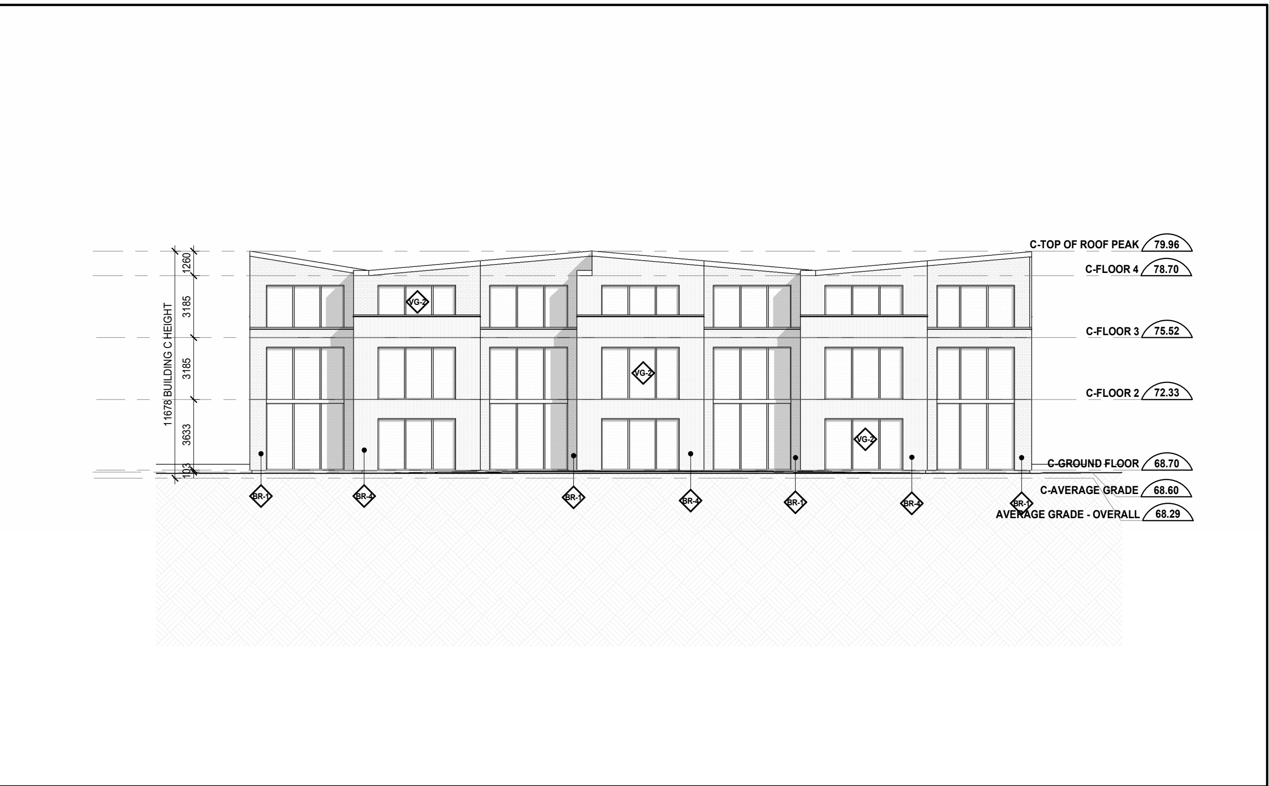
3 Townhouses - South Elevation
