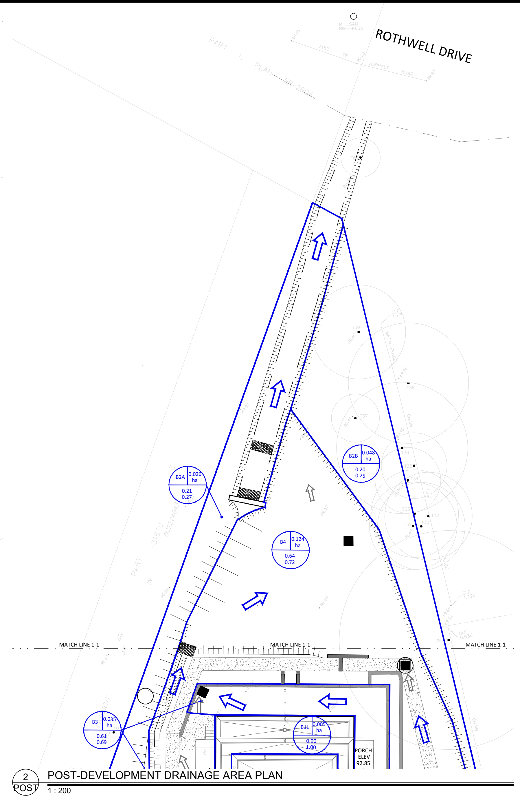
2 POST-DEVELOPMENT DRAINAGE AREA PLAN 1:200
