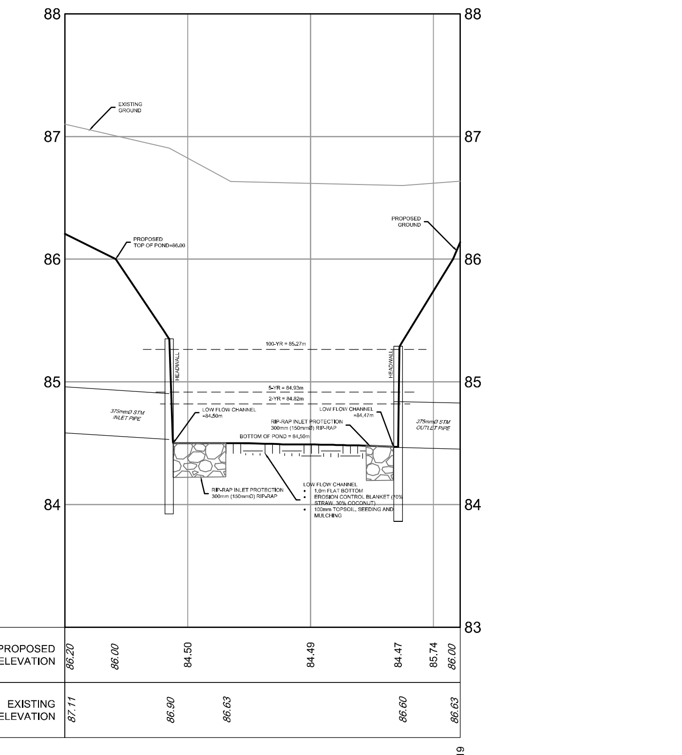
POND CROSS-SECTION A-A
