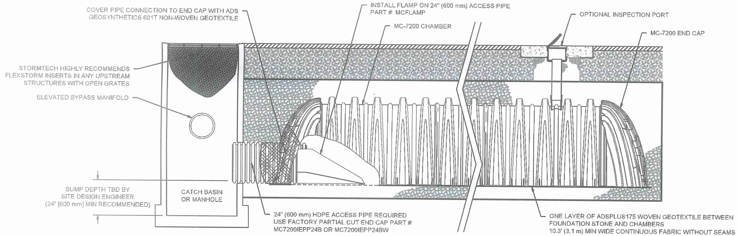
MC-7200 ISOLATOR ROW PLUS DETAIL NTS
