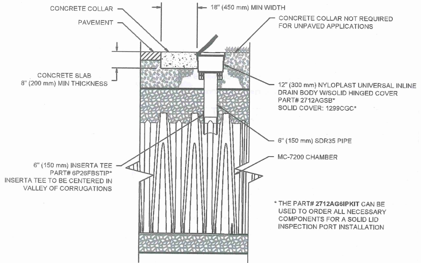
MC-7200 6" (150 mm) INSPECTION PORT DETAIL NTS
