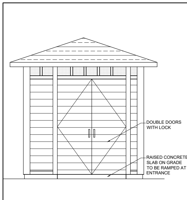
4 GARBAGE ENCLOSURE A-100 FRONT ELEVATION SCALE = 1 : 50
