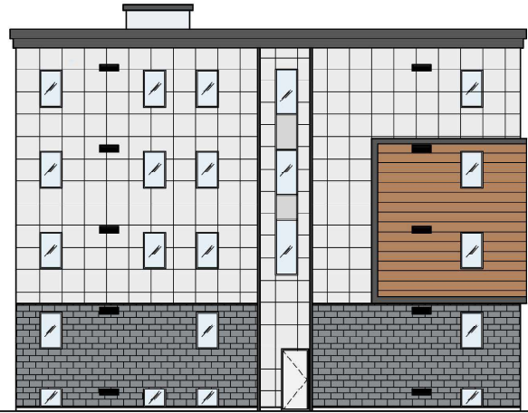
1 NORTH FACADE (FRONT) SCALE = 1/16" = 1'-0"
