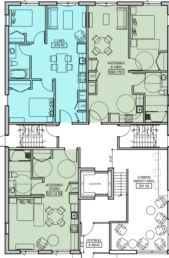
2 FIRST FLOOR PLAN A1 SCALE = 1/16" = 1'-0"
