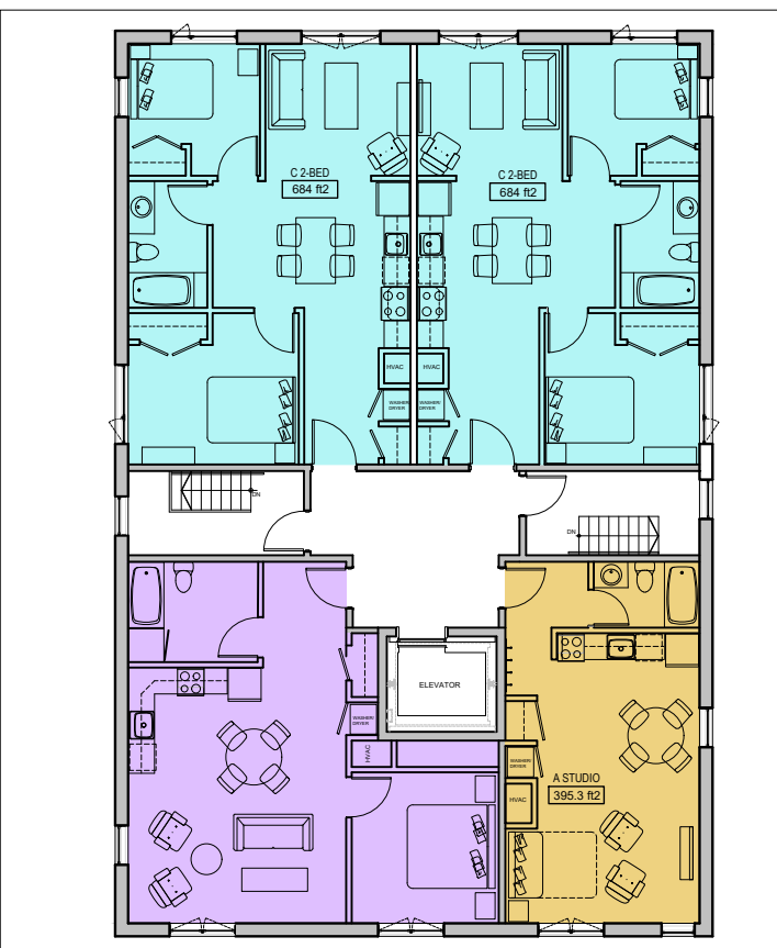
5 FOURTH FLOOR PLAN A1 SCALE = 1/16" = 1'-0"
