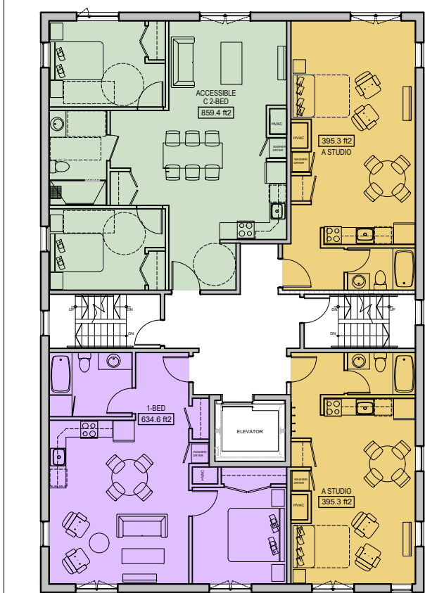
3 SECOND FLOOR PLAN A1 SCALE = 1/16" = 1'-0"
