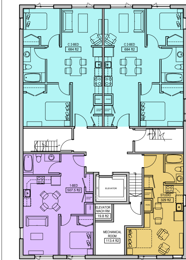
1 BASEMENT FLOOR PLAN A1 SCALE = 1/16" = 1'-0"
