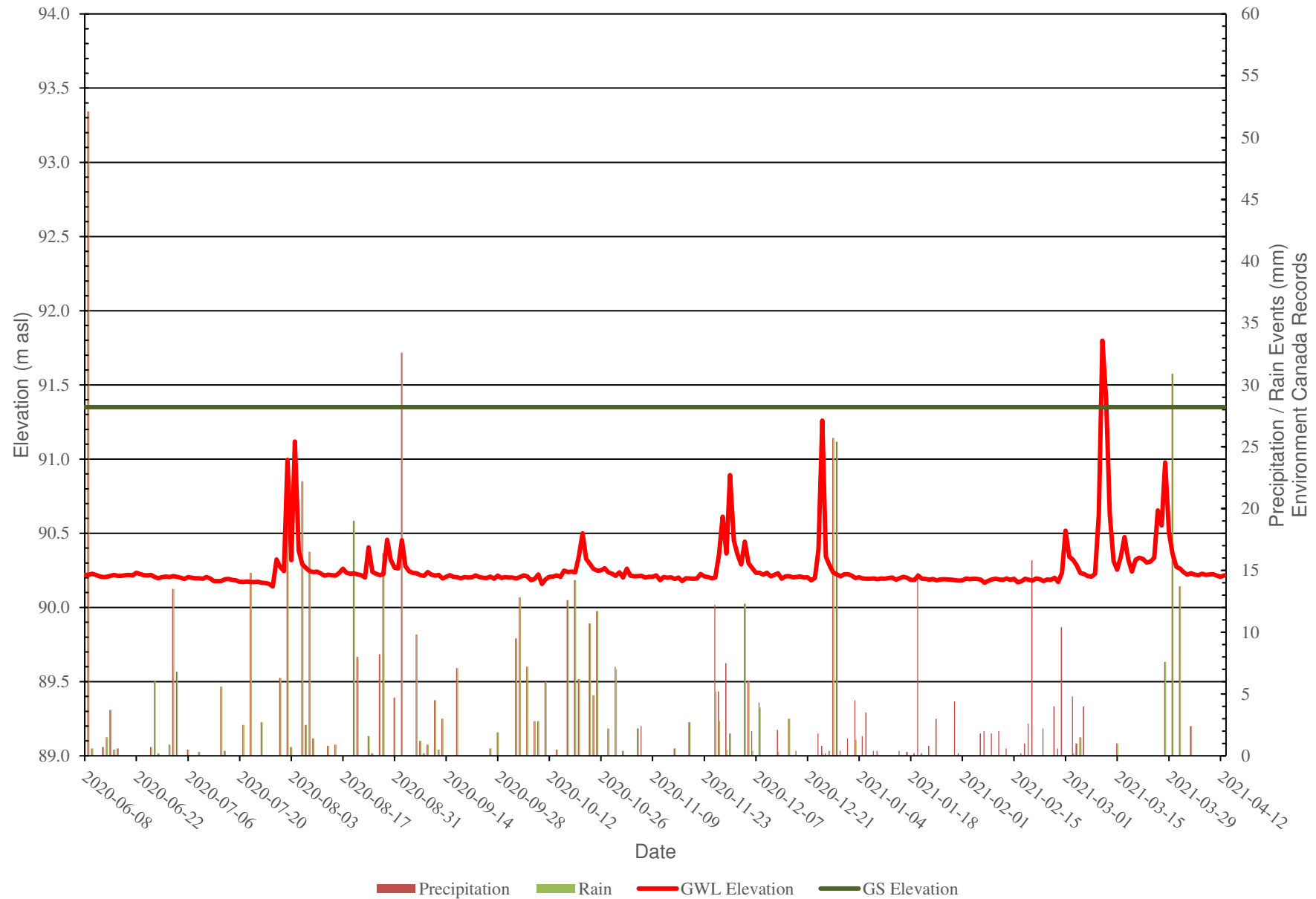
Figure 7: BH17-36 - Groundwater Monitoring Levels vs Precipitation Data
