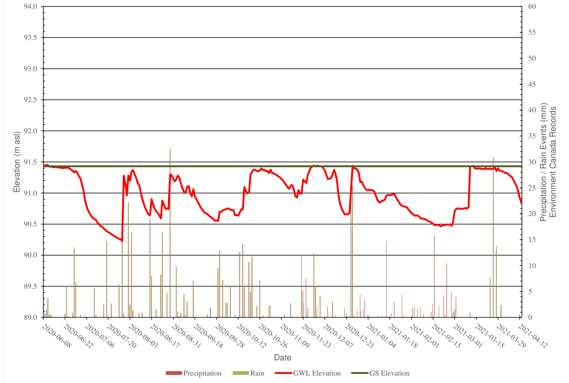
Figure 11: BH17-52 - Groundwater Monitoring Levels vs Precipitation Data
