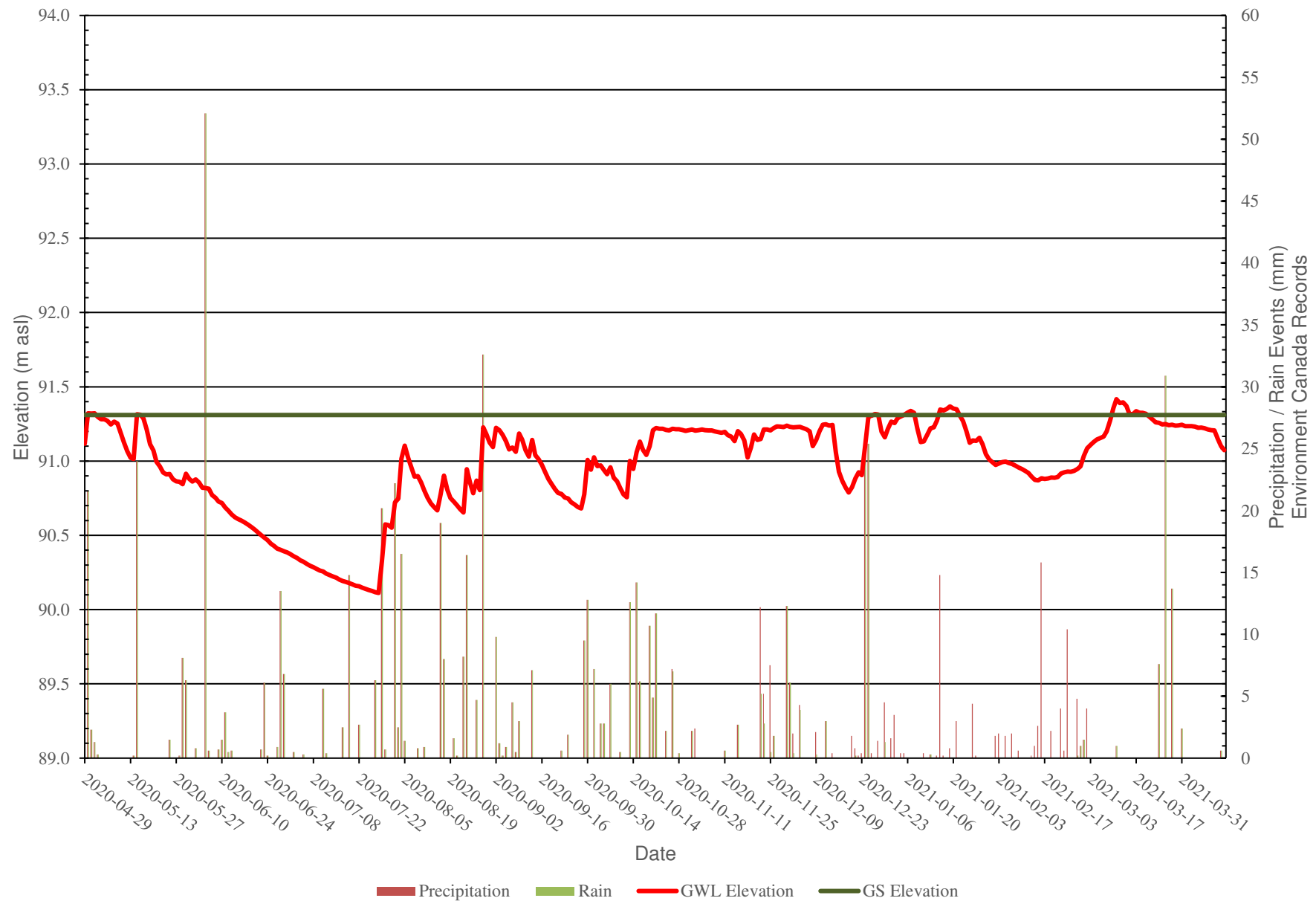
Figure 17: BH18-22s - Groundwater Monitoring Levels vs Precipitation Data
