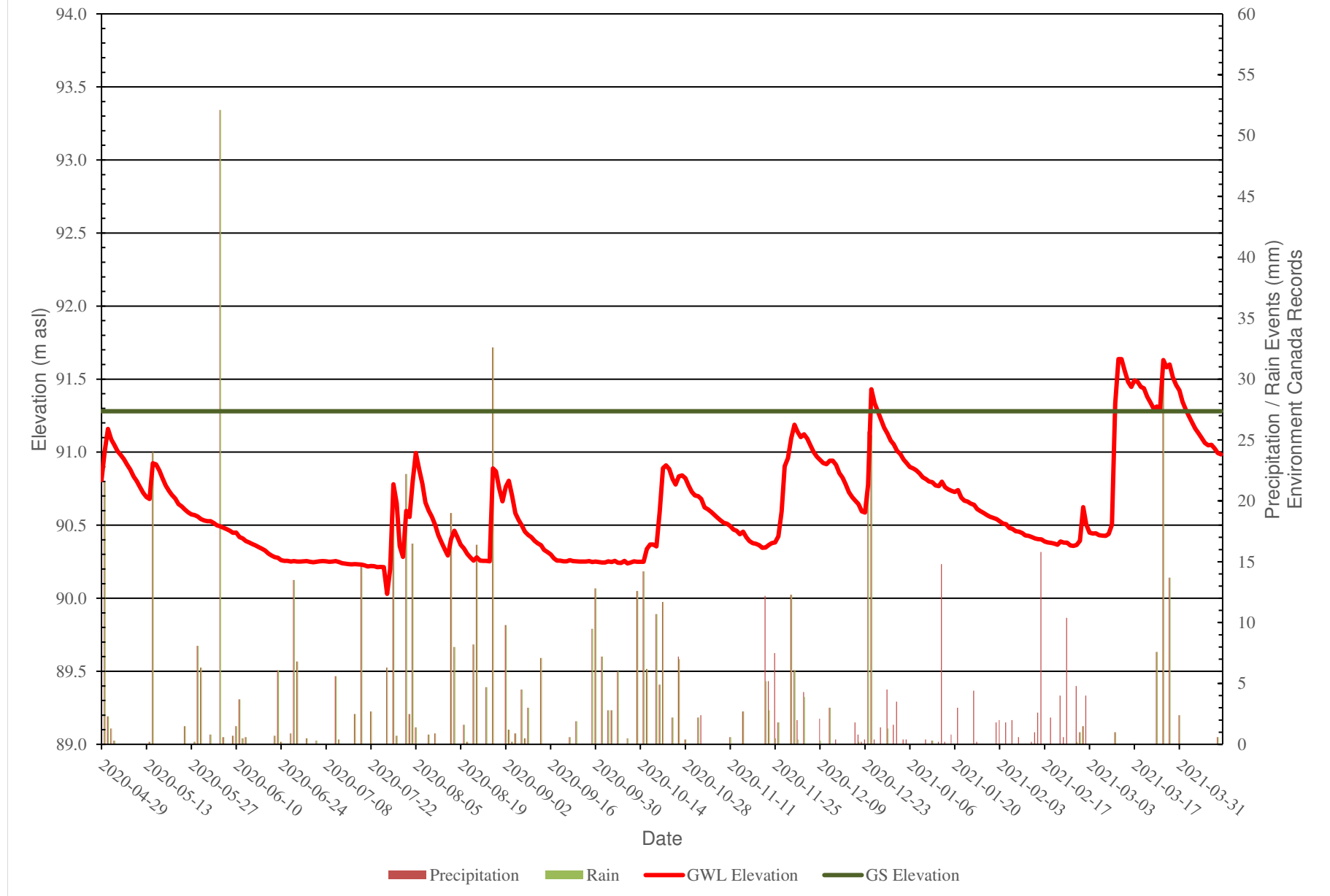
Figure 12: BH18-04s - Groundwater Monitoring Levels vs Precipitation Data
