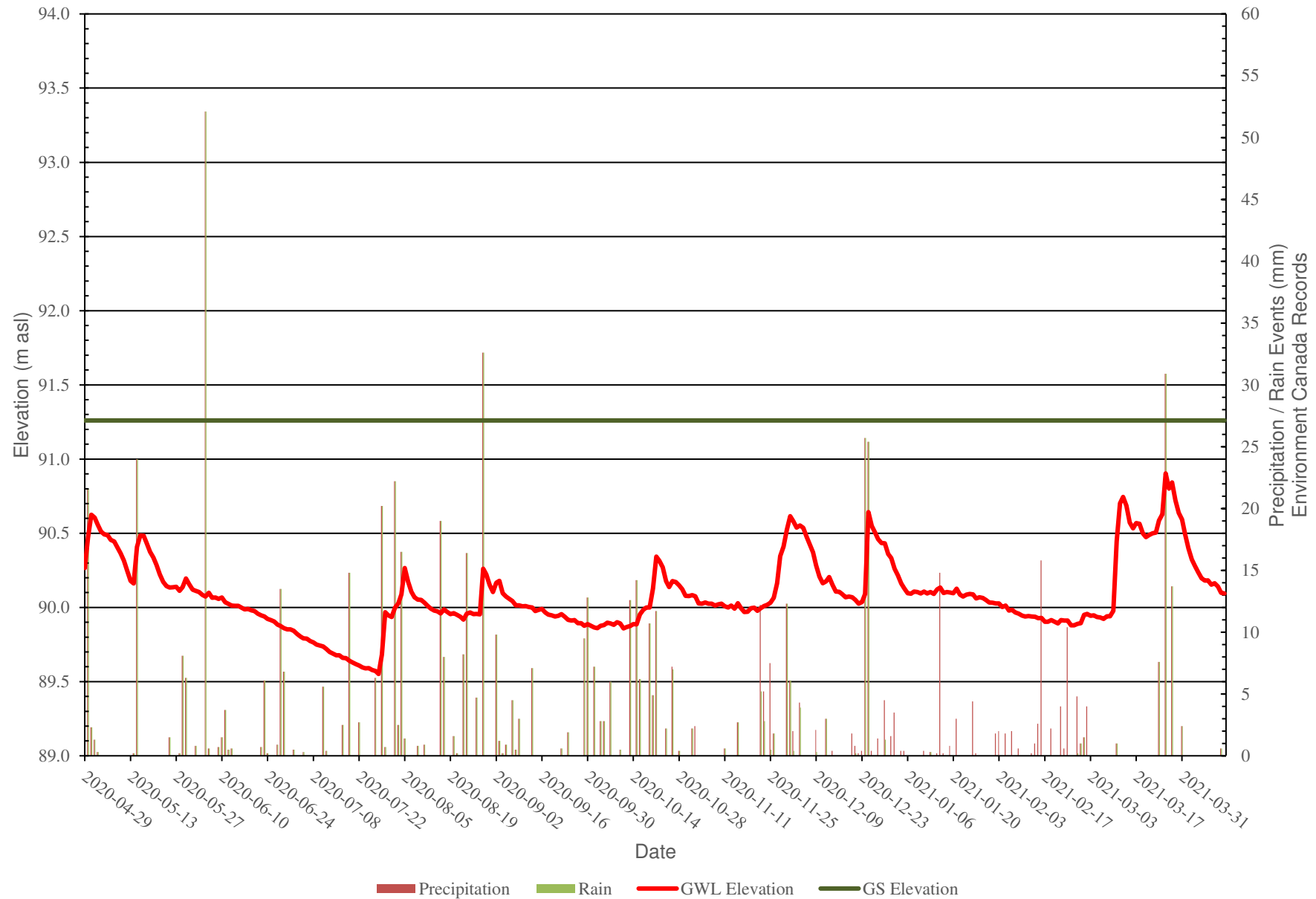
Figure 16: BH18-19 - Groundwater Monitoring Levels vs Precipitation Data
