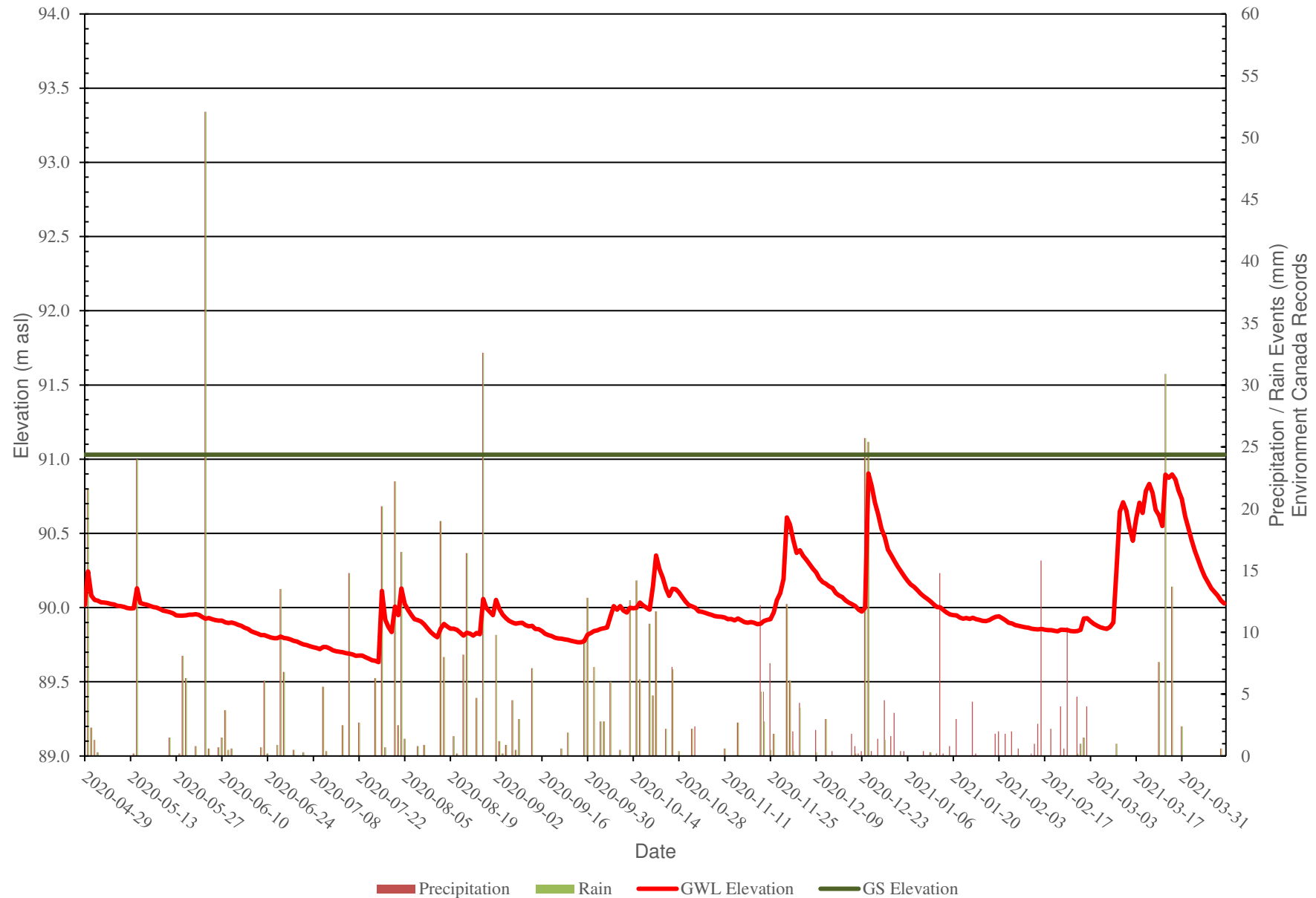
Figure 3: BH17-20s - Groundwater Monitoring Levels vs Precipitation Data
