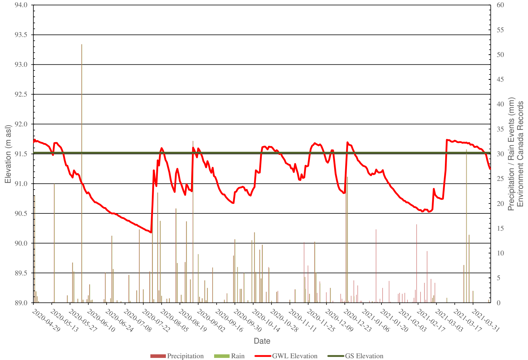
Figure 9: BH17-43 - Groundwater Monitoring Levels vs Precipitation Data
