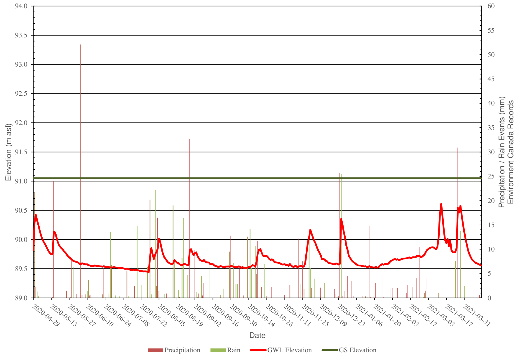
Figure 6: BH17-32s - Groundwater Monitoring Levels vs Precipitation Data
