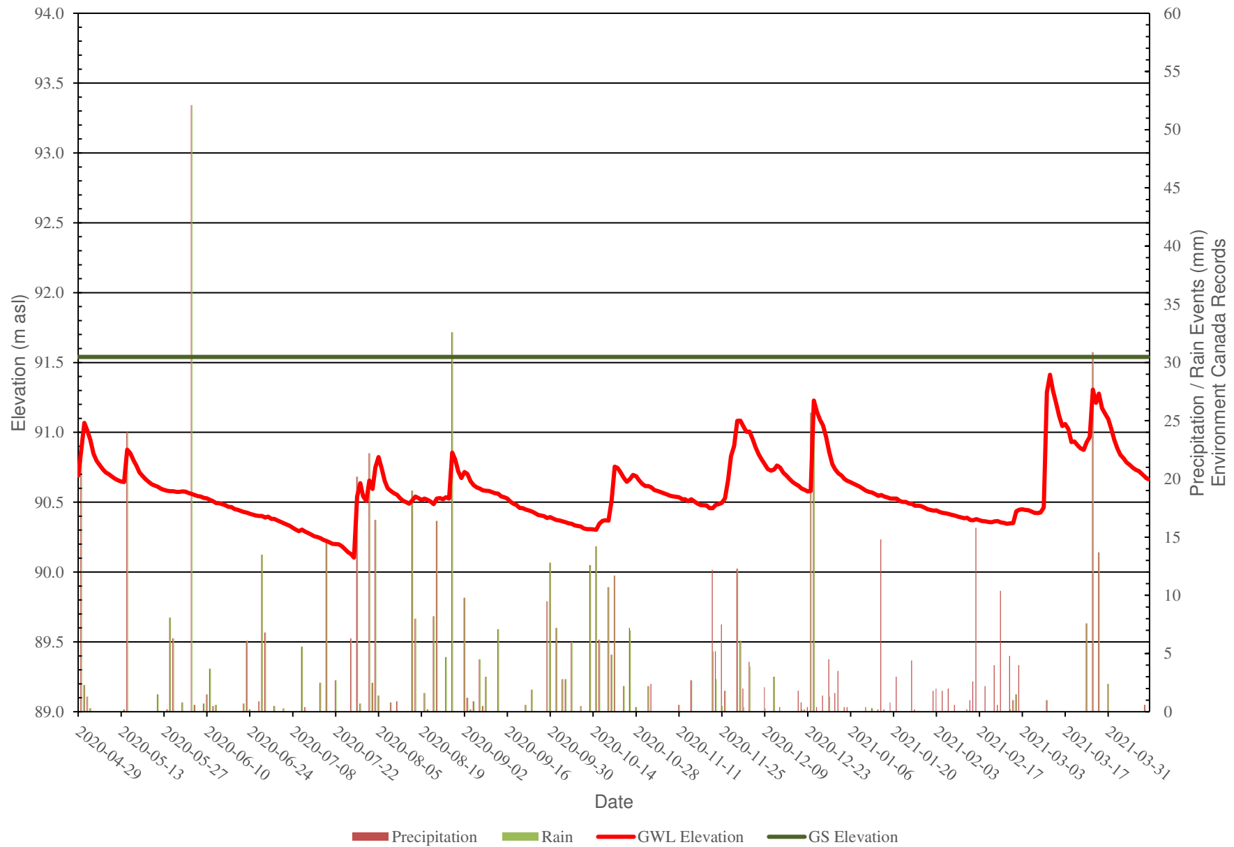
Figure 5: BH17-26 - Groundwater Monitoring Levels vs Precipitation Data
