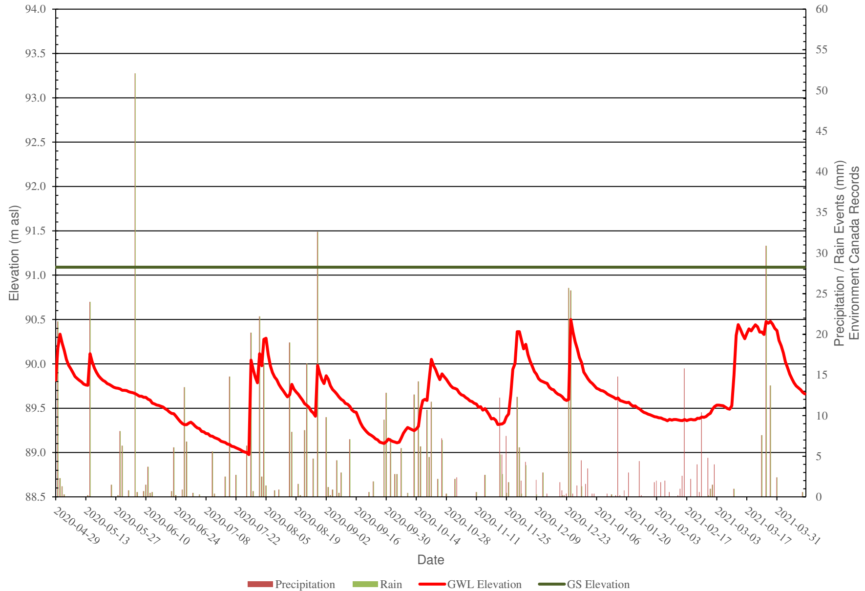
Figure 4: BH17-25s - Groundwater Monitoring Levels vs Precipitation Data
