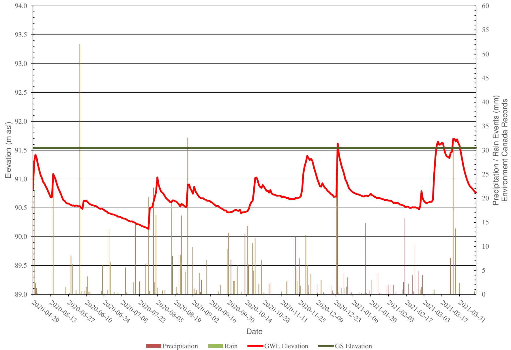
Figure 15: BH18-18s - Groundwater Monitoring Levels vs Precipitation Data
