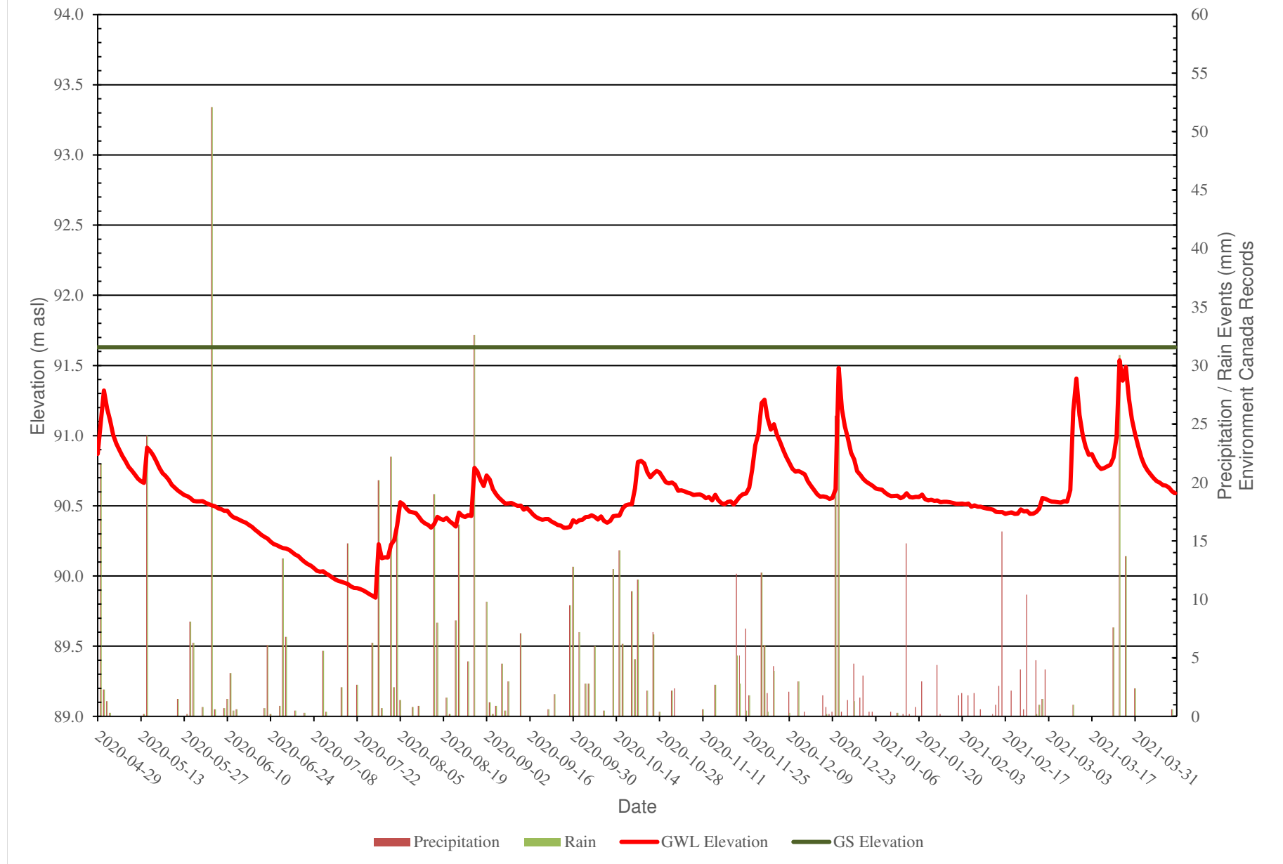
Figure 10: BH17-46s - Groundwater Monitoring Levels vs Precipitation Data
