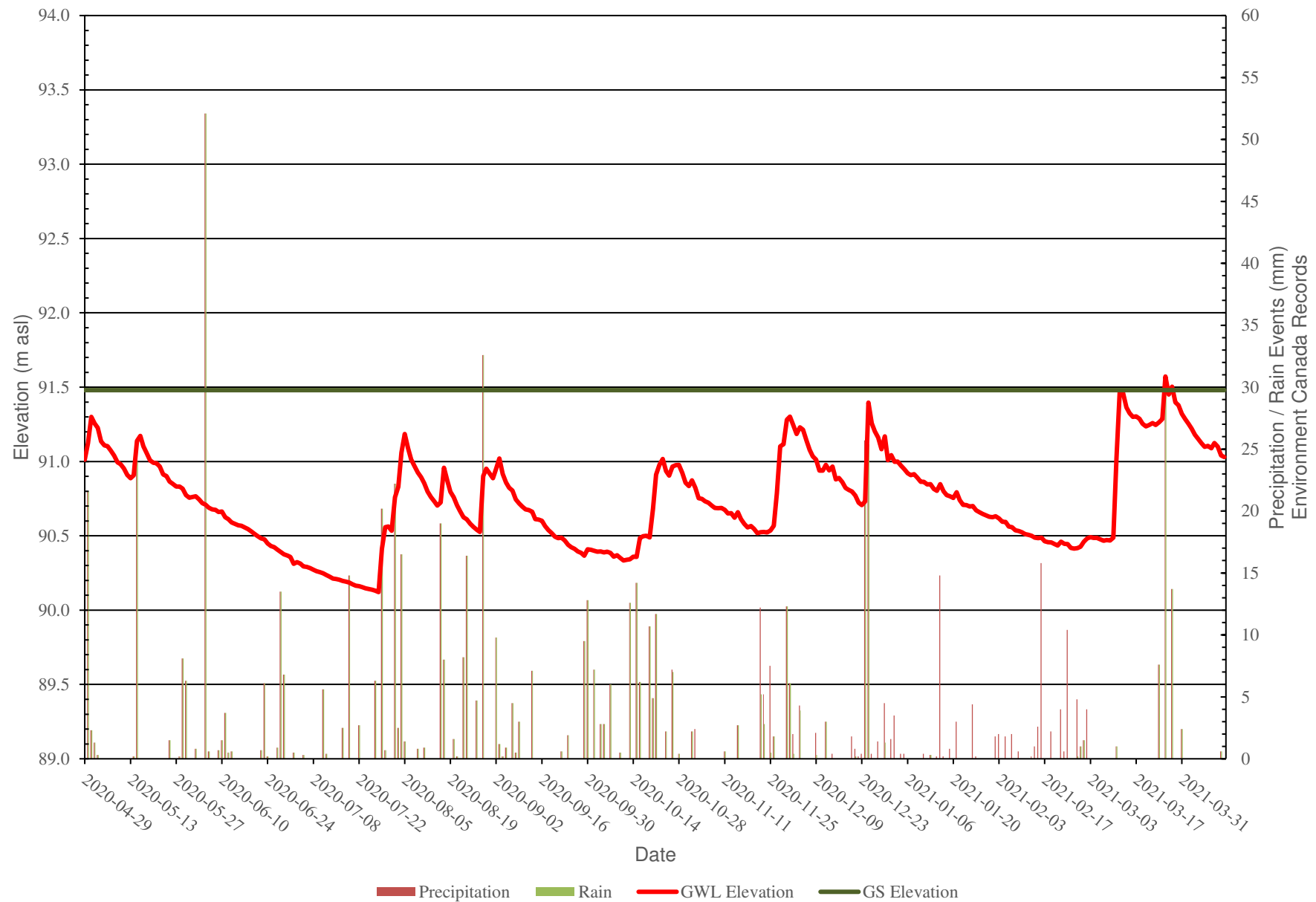
Figure 14: BH18-08 - Groundwater Monitoring Levels vs Precipitation Data
