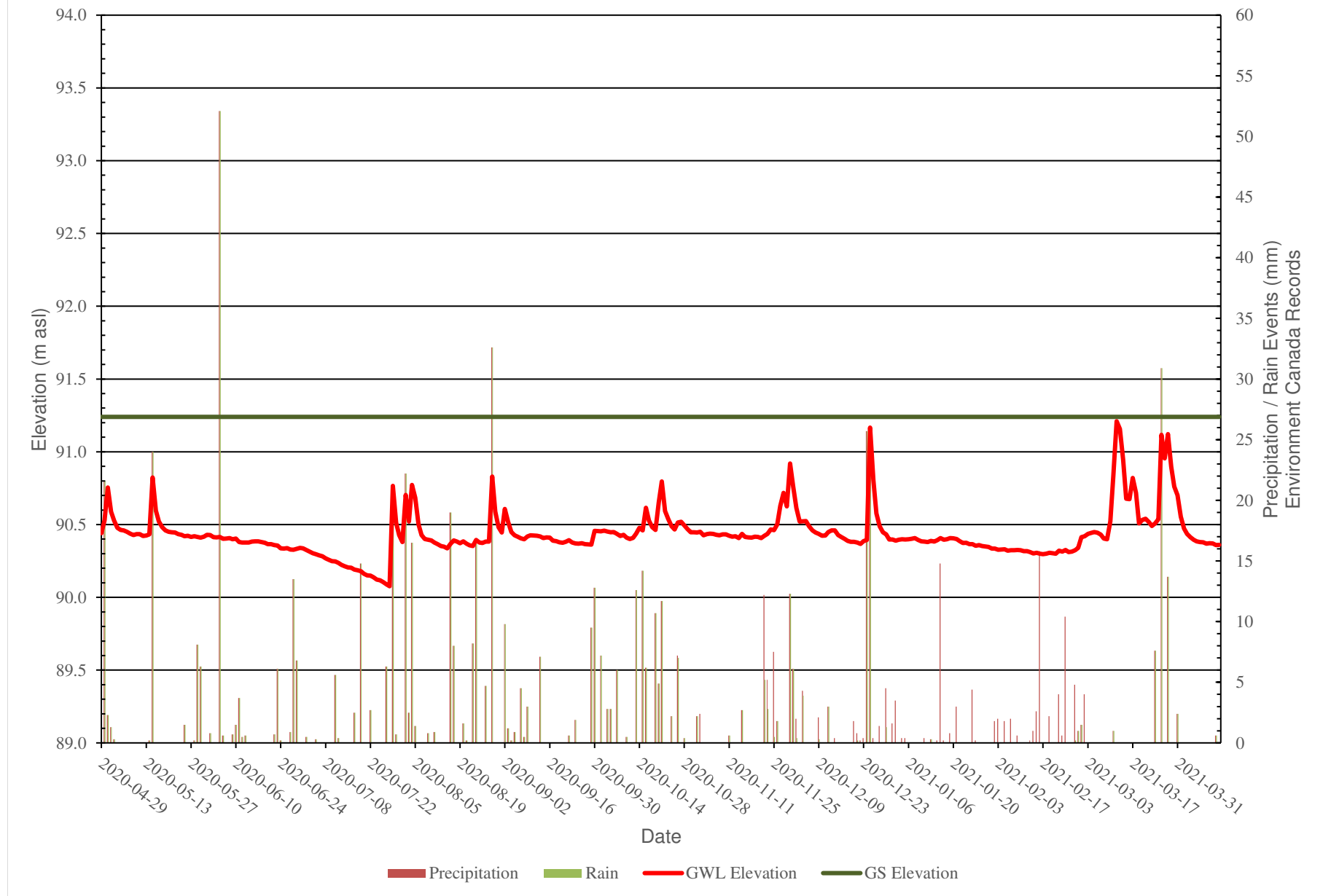
Figure 8: BH17-38s - Groundwater Monitoring Levels vs Precipitation Data
