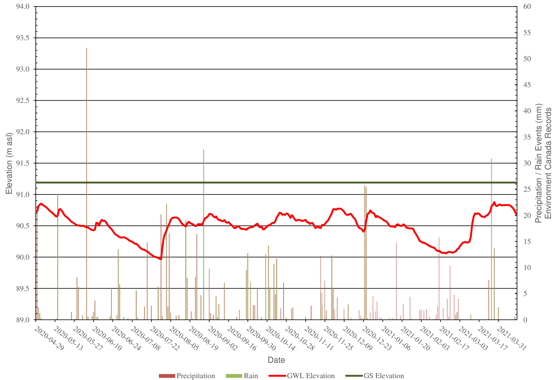
Figure 1: BH17-11 - Groundwater Monitoring Levels vs Precipitation Data
