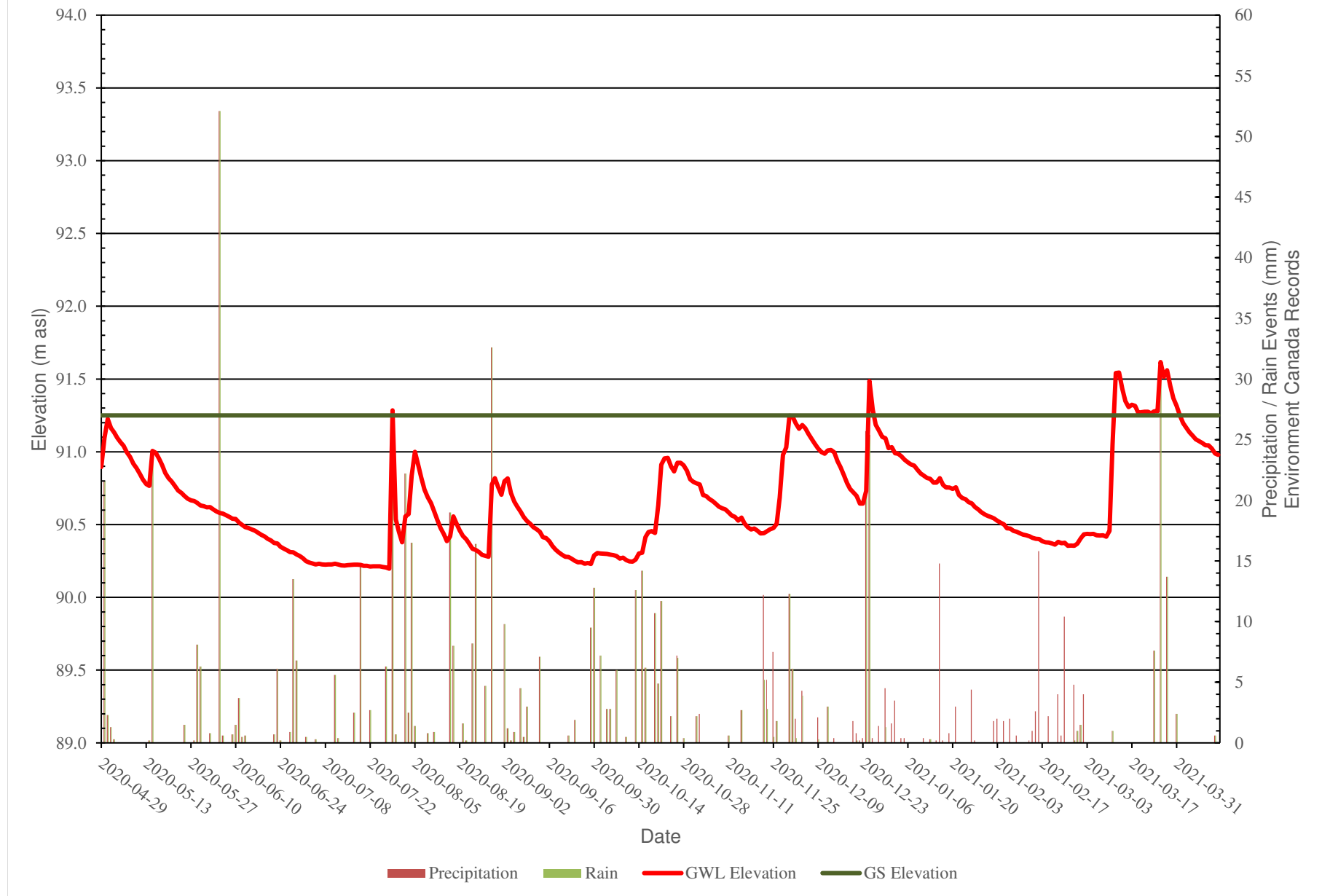
Figure 13: BH18-06 - Groundwater Monitoring Levels vs Precipitation Data
