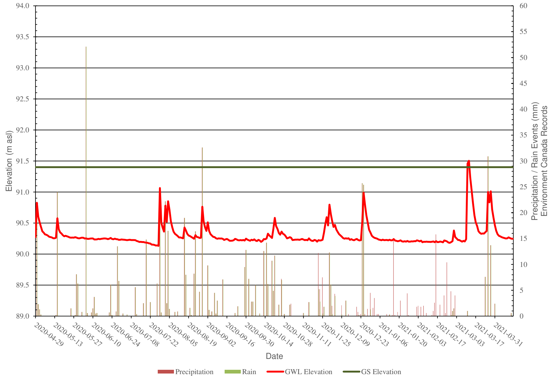
Figure 2: BH17-18s - Groundwater Monitoring Levels vs Precipitation Data
