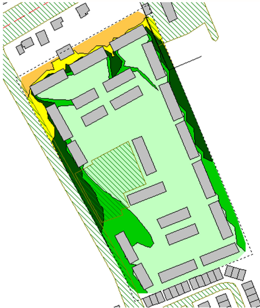
FIGURE 7: NIGHTTIME TRAFFIC NOISE CONTOURS (1.5 M ABOVE GRADE)
