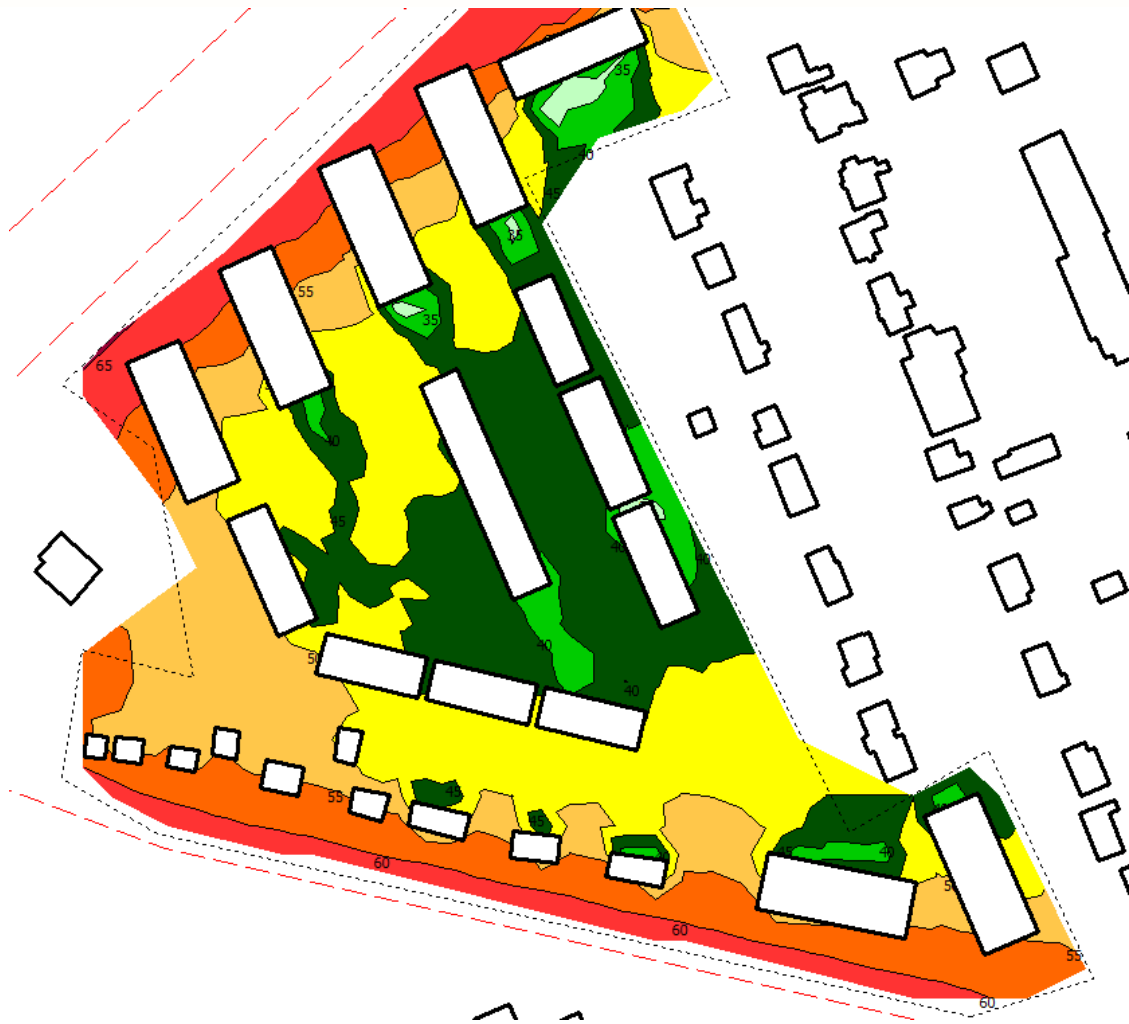
FIGURE 5: NIGHTTIME NOISE CONTOURS AT 1.5 M AGL
