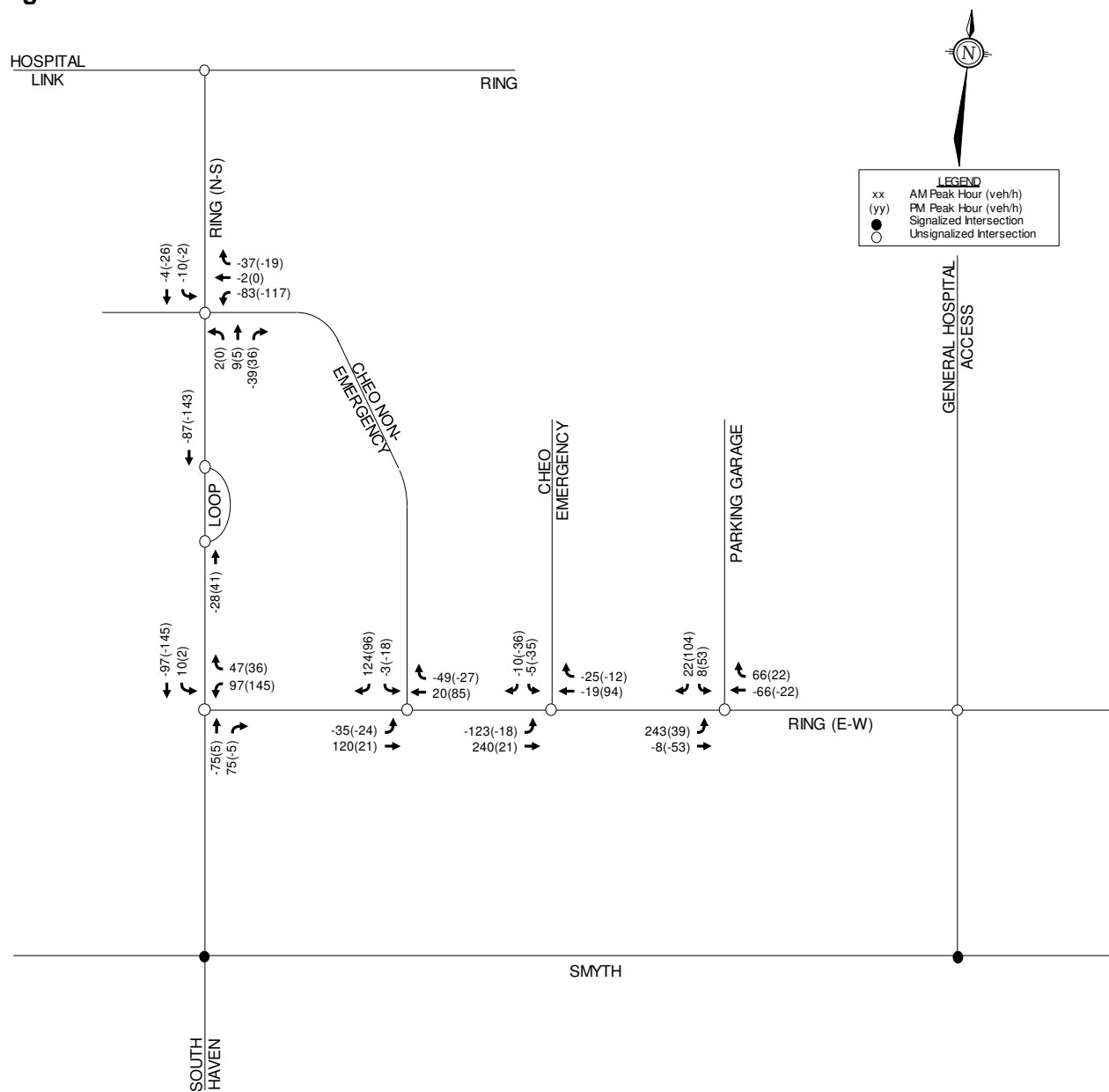
Figure 15: Net Relocated Traffic
