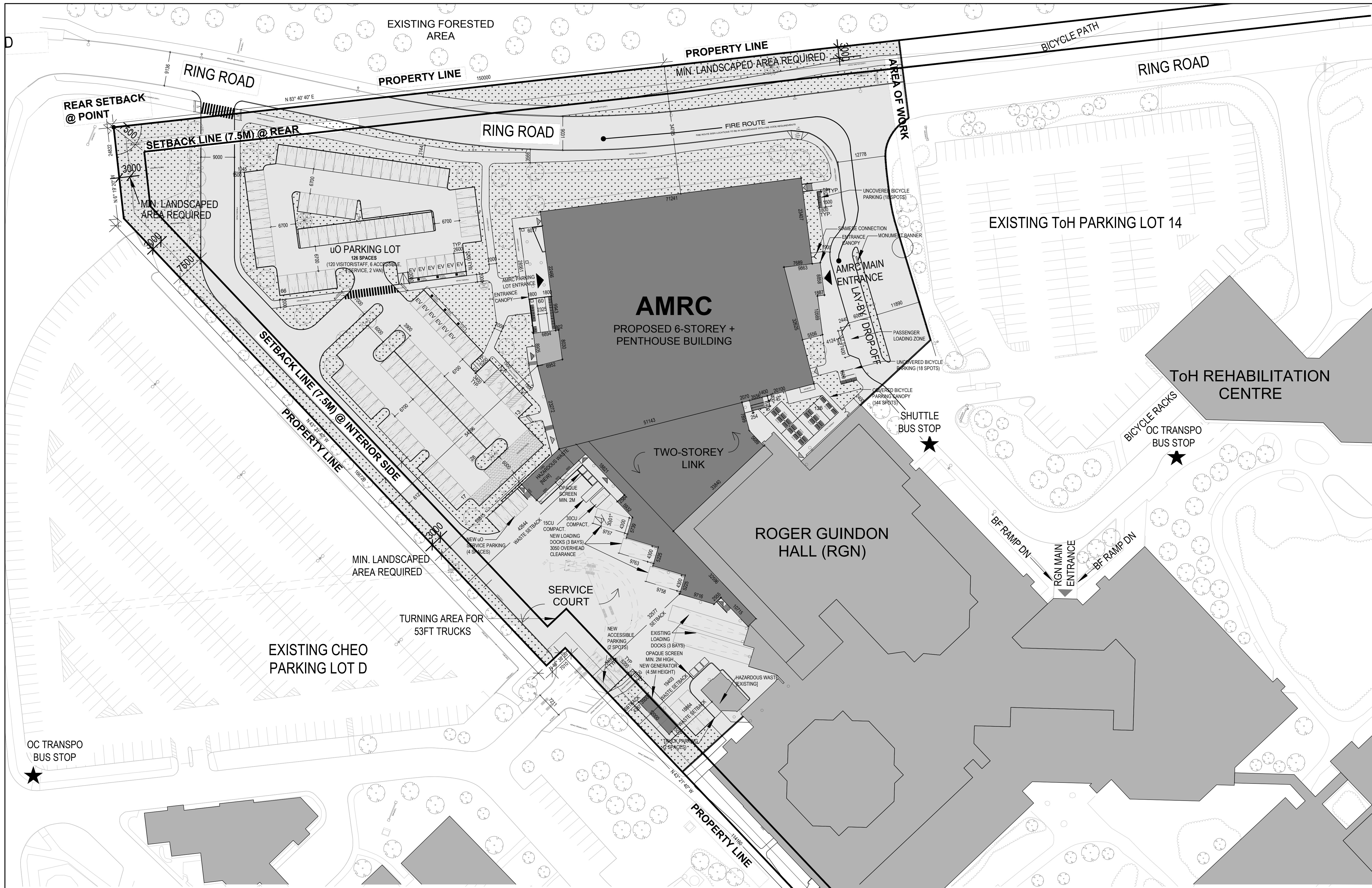
SITE PLAN - PROPOSED 1:500
