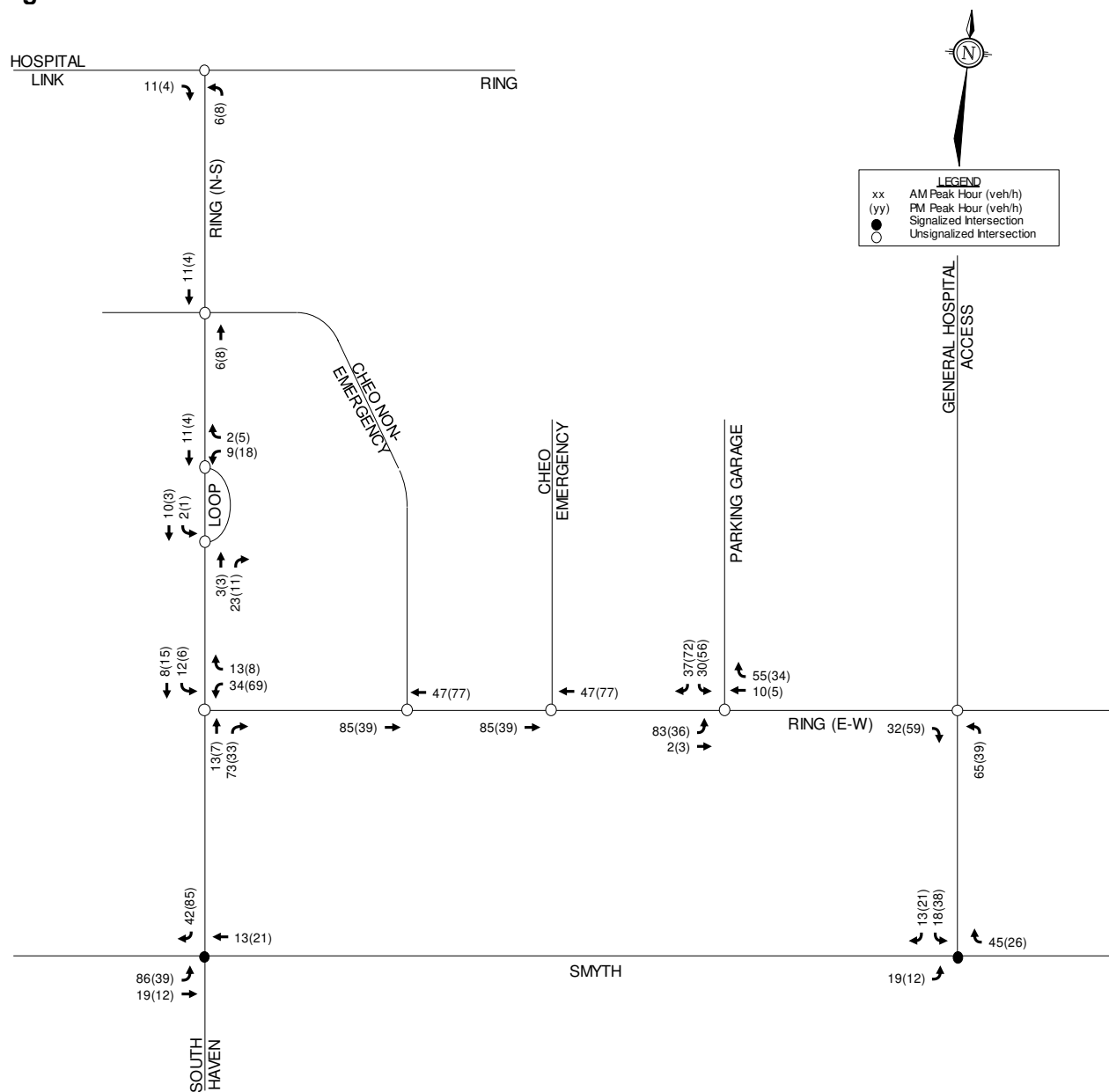
Figure 11: Site-Generated Traffic Volumes
