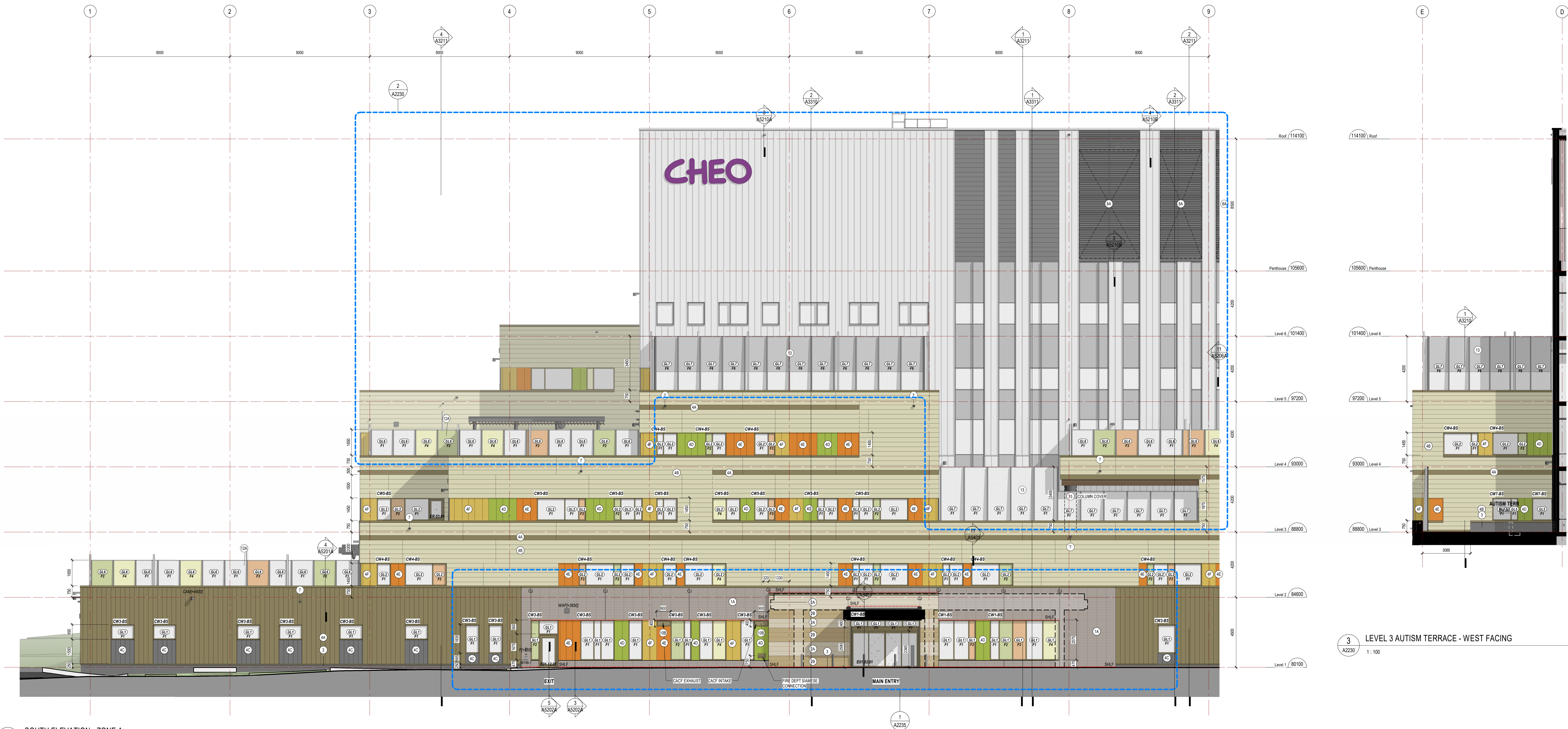
1 SOUTH ELEVATION - ZONE A A2230 1:100
