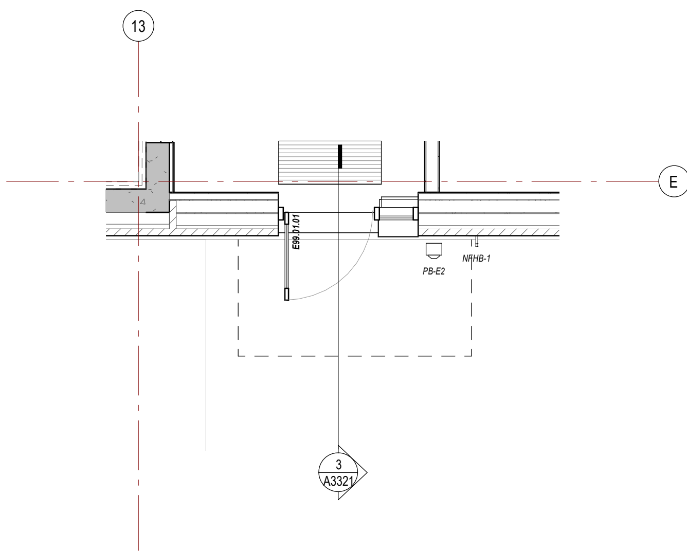
4 L1 STAFF ENTRANCE CANOPY - PLAN A1801 1:50
