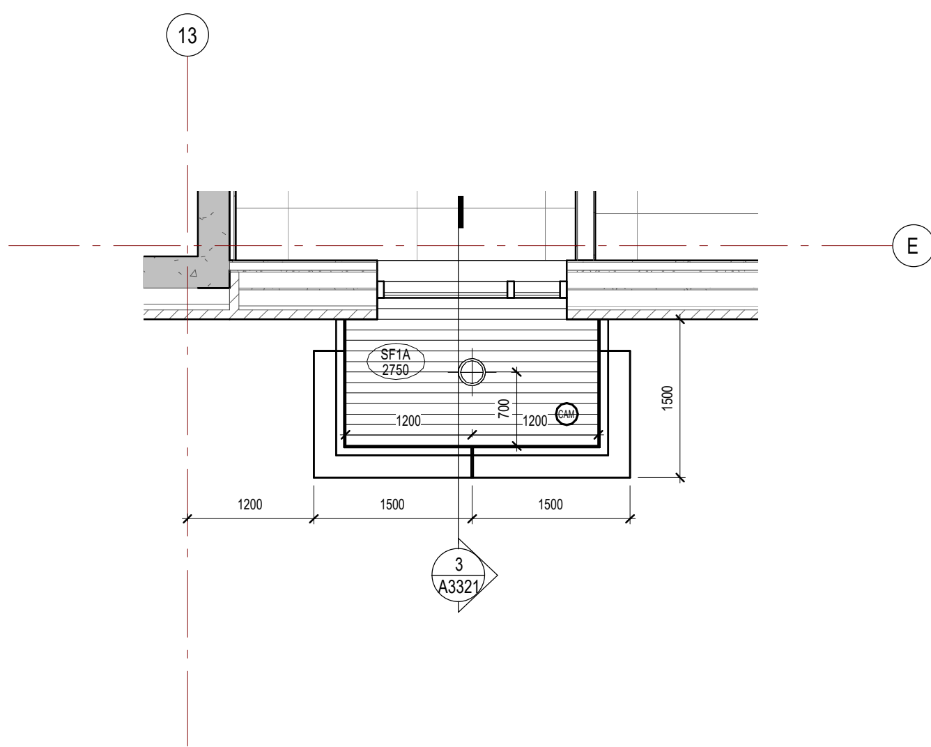
5 L1 STAFF ENTRANCE CANOPY - RCP A1801 1:50
