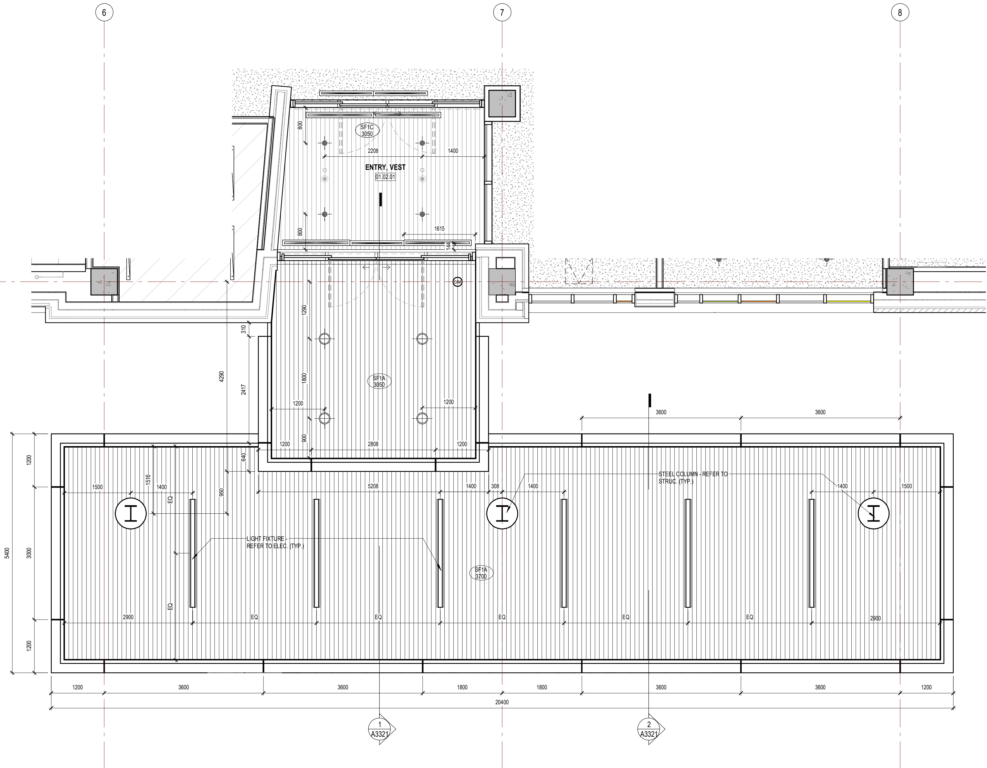
2 L1 MAIN CANOPY - RCP A1801 1:50
