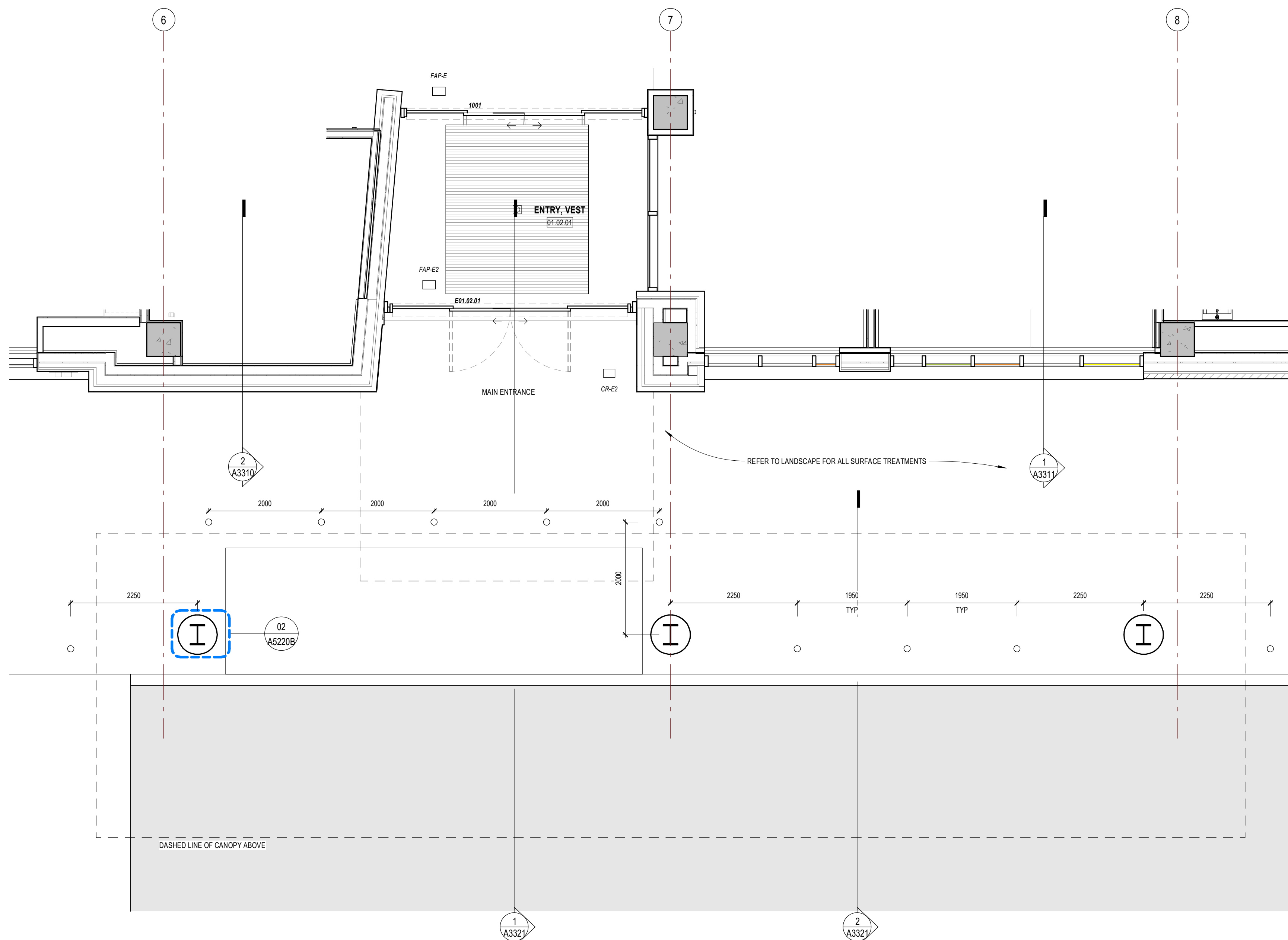
1 L1 MAIN CANOPY - PLAN A1801 1:50
