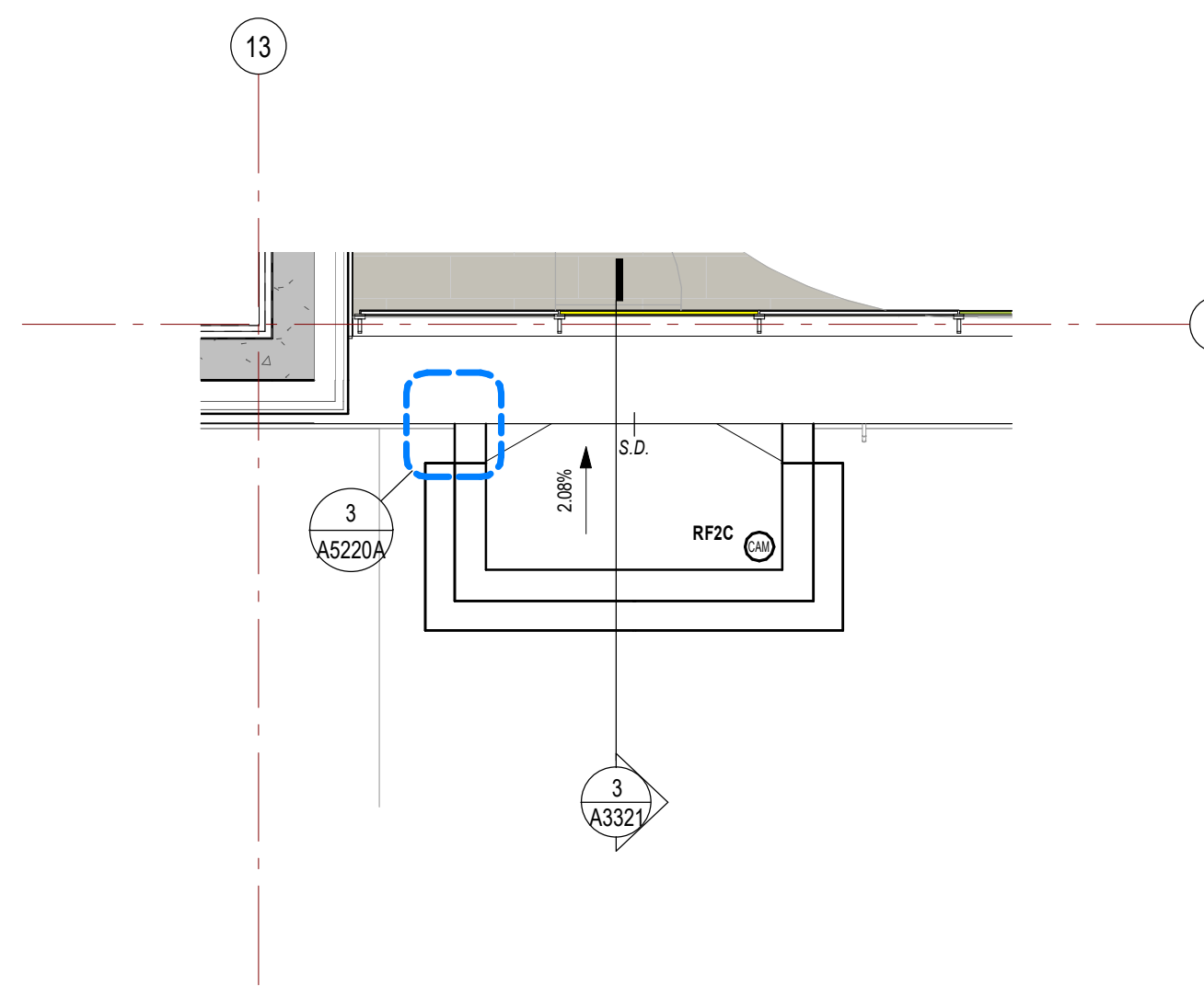
6 L1 STAFF ENTRANCE CANOPY - ROOF PLAN A1801 1:50
