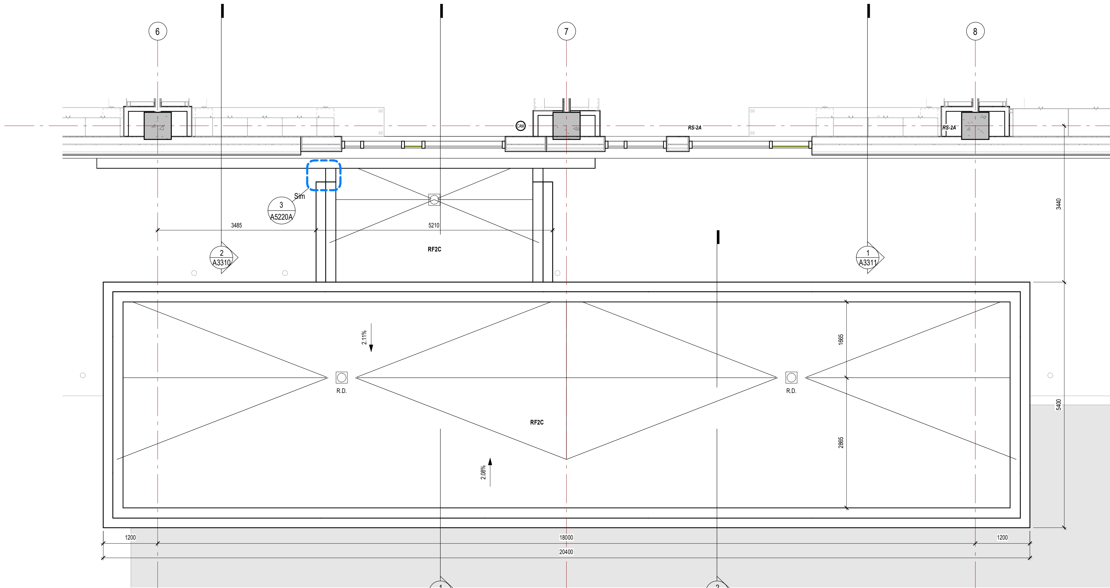
3 L1 MAIN CANOPY - ROOF PLAN A1801 1:50
