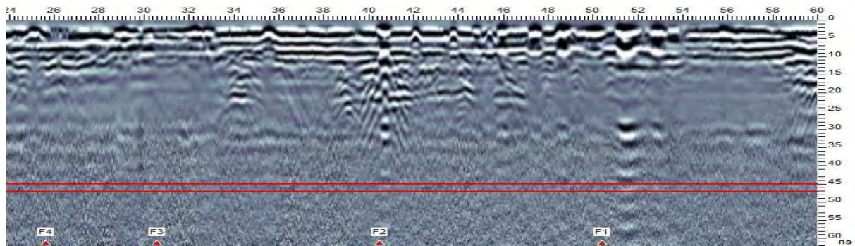
Figure 18: Example of GPR Profiles - Grid XLine3
