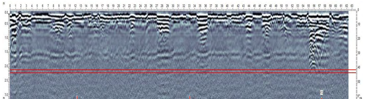
Figure 16: Example of GPR Profiles - Grid3 XLine2
