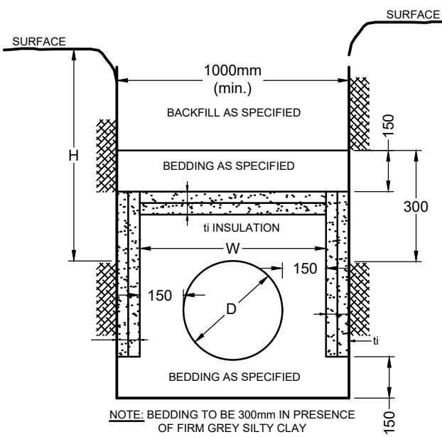
INSULATION DETAIL FOR SHALLOW SEWERS & WATERMAIN N.T.S.
