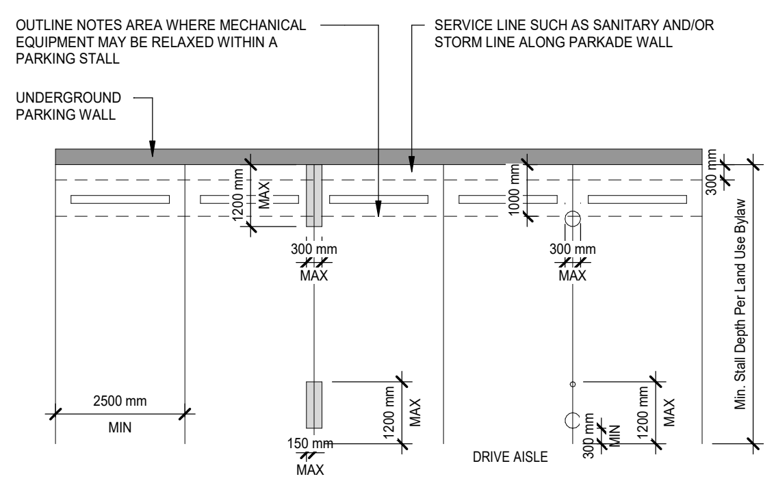
2 VOLUMETRIC ENCROACHMENT PLAN DIAGRAM (TYPICAL) DP20-00-01 SCALE: 1 : 100
