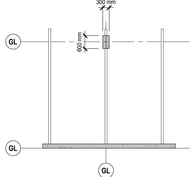
4 TYPICAL COLUMN MEASUREMENTS DP20-00-01 SCALE: 1 : 100
