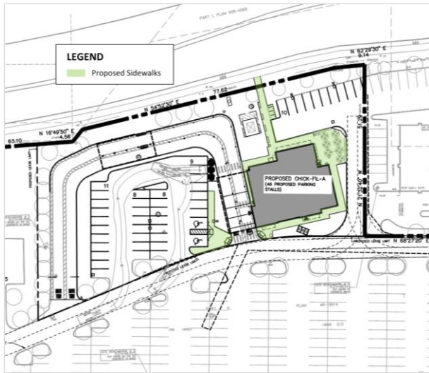
Figure 17: Overall Site Plan
