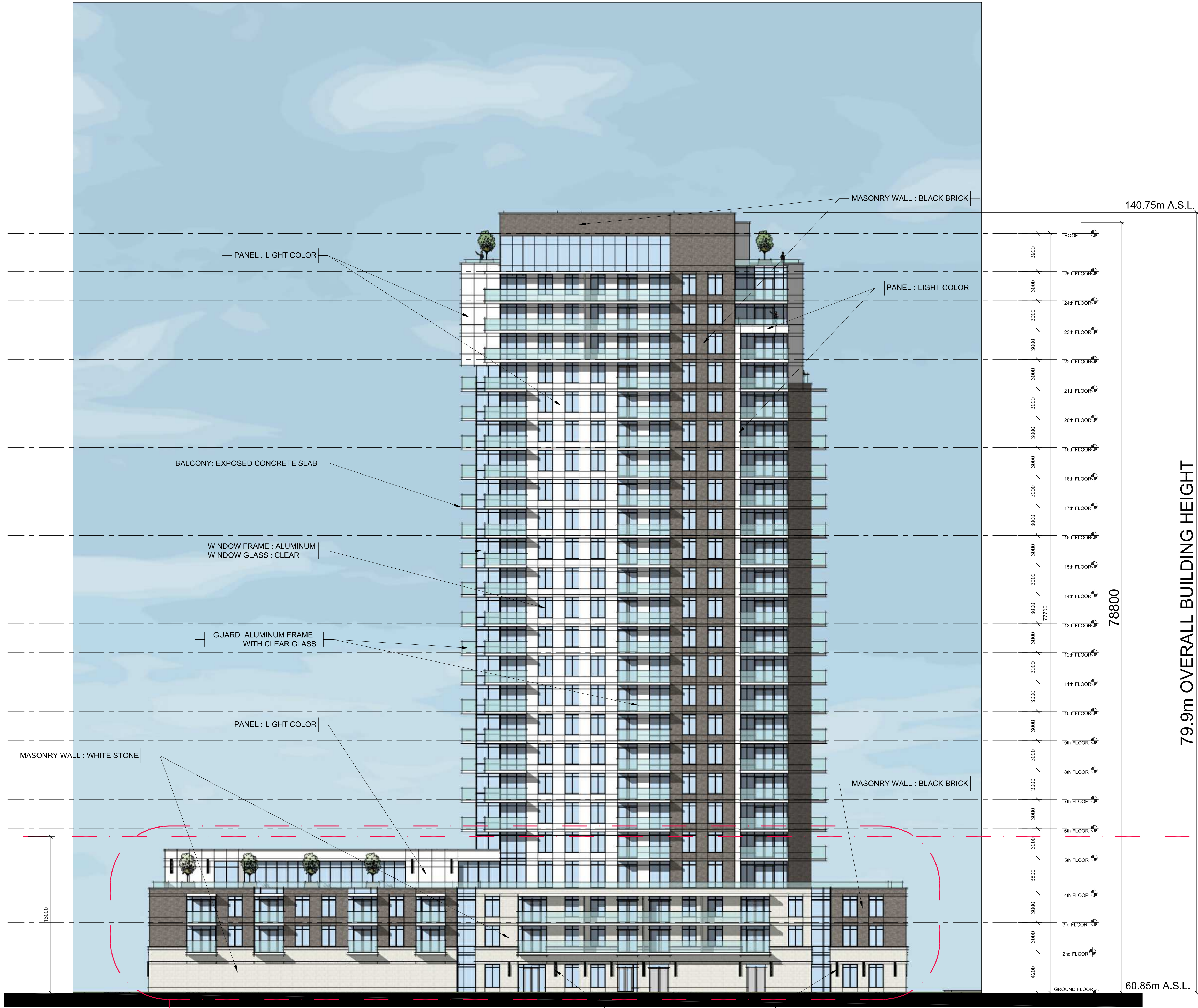
WEST ELEVATION
