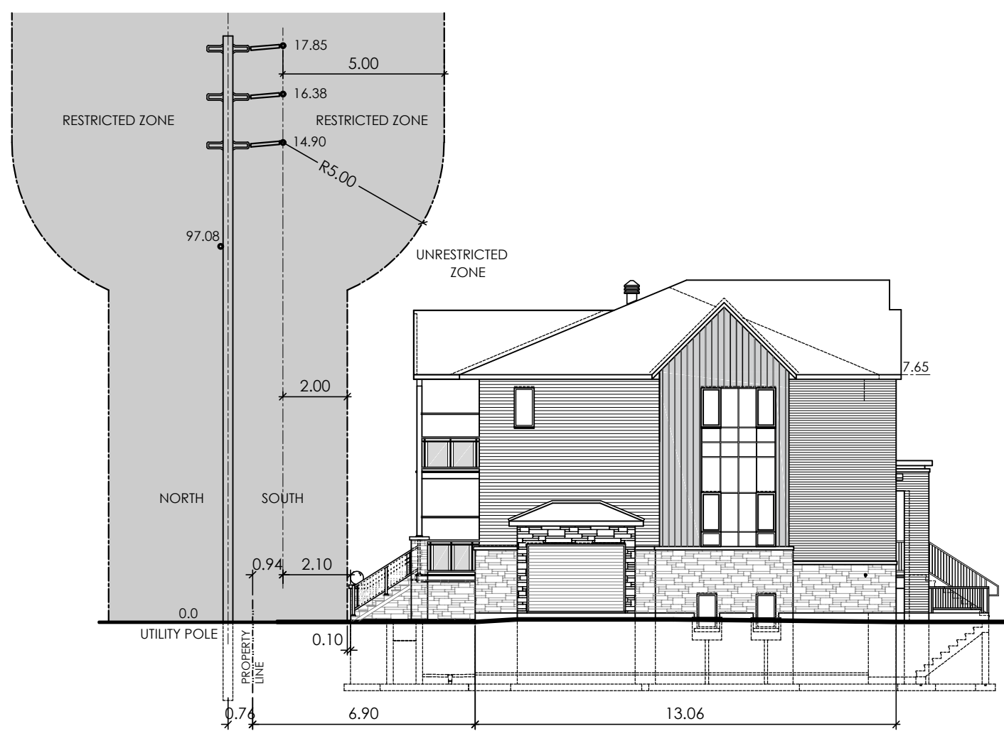
HYDRO CLEARANCE SKETCH BLOCK 5 - WEST SIDE ELEVATION SCALE 1:200 NOTE: HEIGHTS OF HYDRO WIRES TO BE CONFIRMED FOR BLOCK 140.
