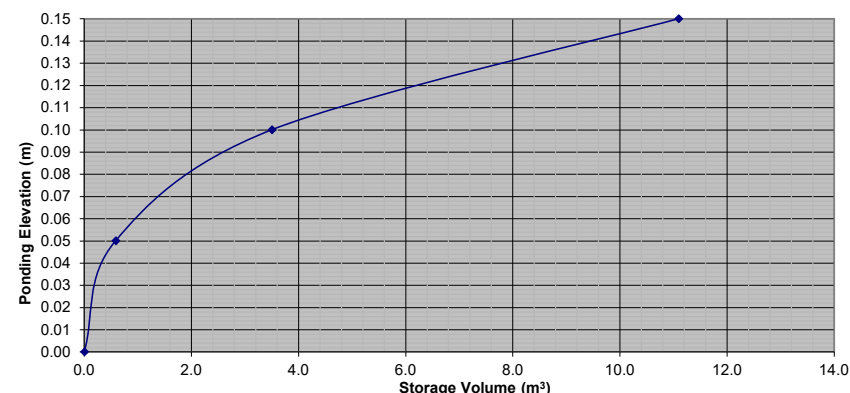
Stage Storage Curve: Area A-5 Controlled Roof Drain #14
