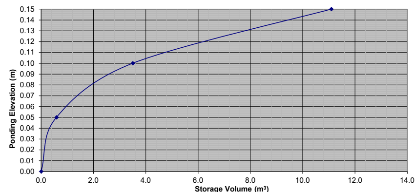
Stage Storage Curve: Area A-5 Controlled Roof Drain #16
