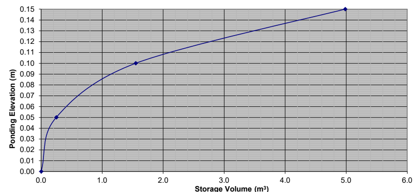
Stage Storage Curve: Area A-5 Controlled Roof Drain #9
