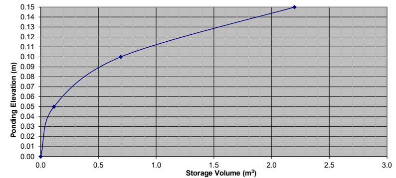
Stage Storage Curve: Area A-6 Controlled Roof Drain #5
