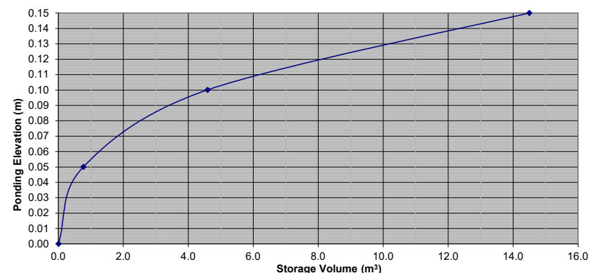
Stage Storage Curve: Area A-4 Controlled Roof Drain #1
