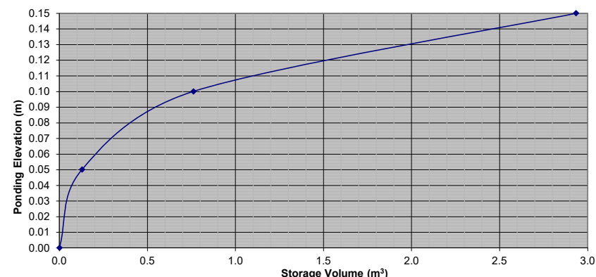
Stage Storage Curve: Area A-5 Controlled Roof Drain #3
