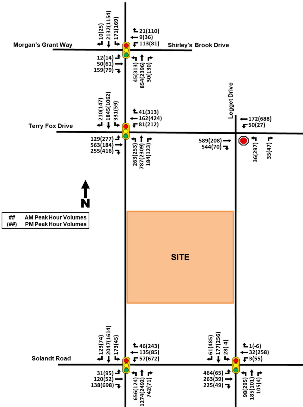
Figure 10 - 2032 Future Background Volumes
