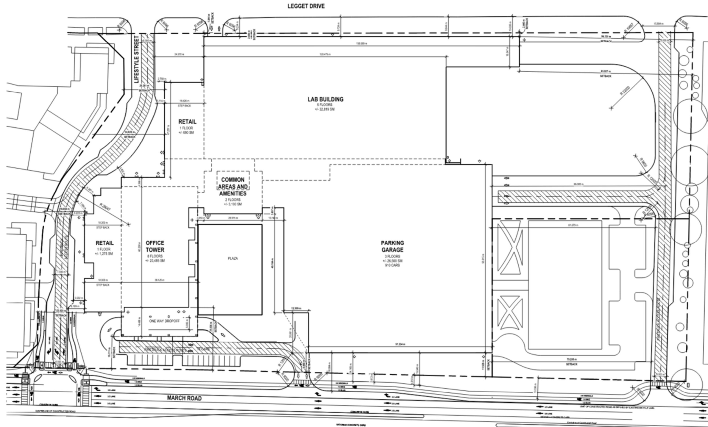
Figure 2 - Proposed Development Site Plan
