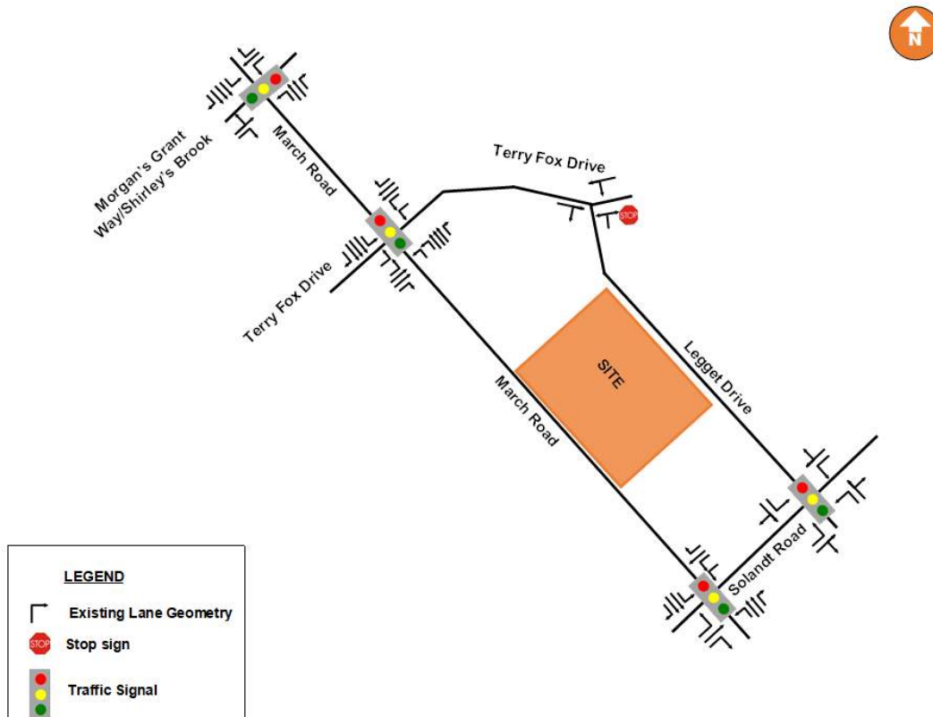
Figure 3 - Existing Lane Configuration and Traffic Control
