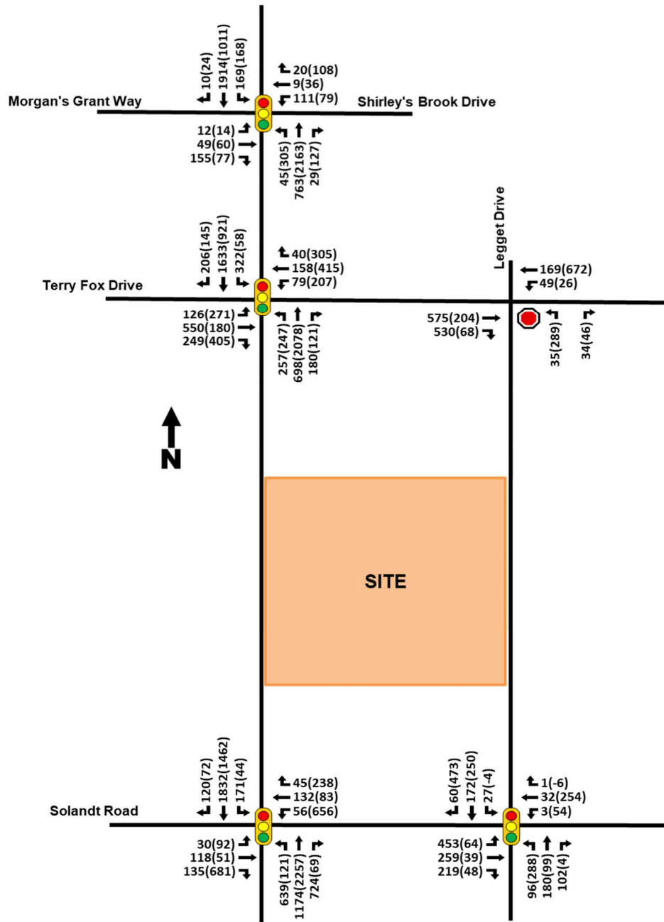
Figure 9 - 2027 Future Background Volumes
