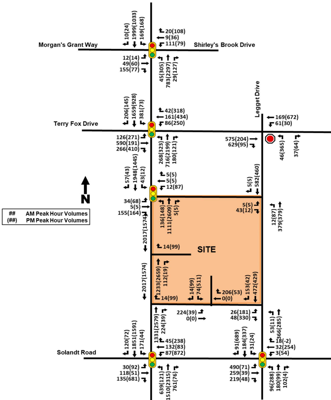
Figure 11 - 2027 Future Total Traffic Volumes
