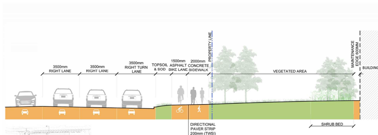
Figure 17 – Conceptual March Road Cross-Section
