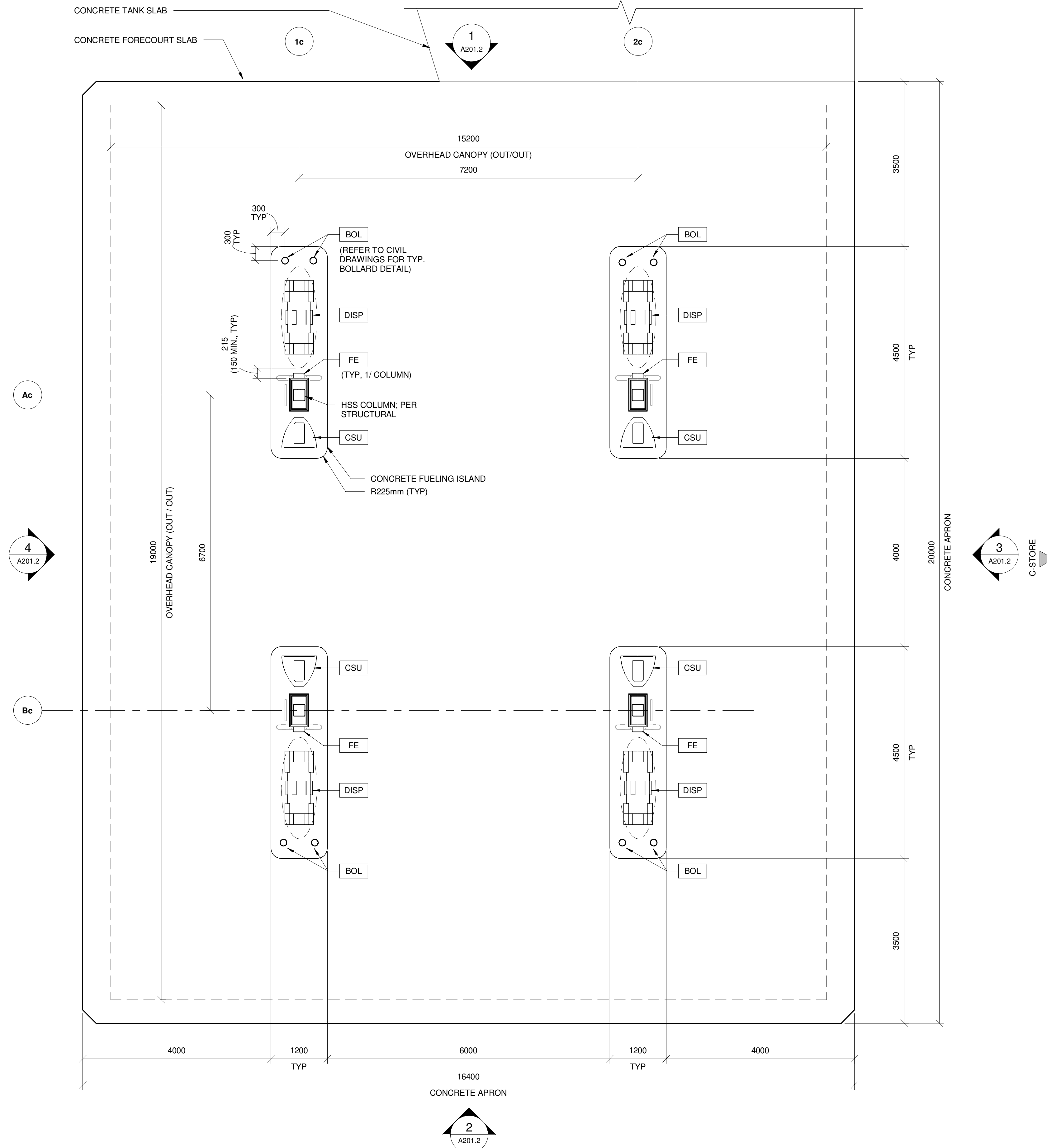
1 A101.2 | FUEL PUMP PLAN Scale: 1 : 50
