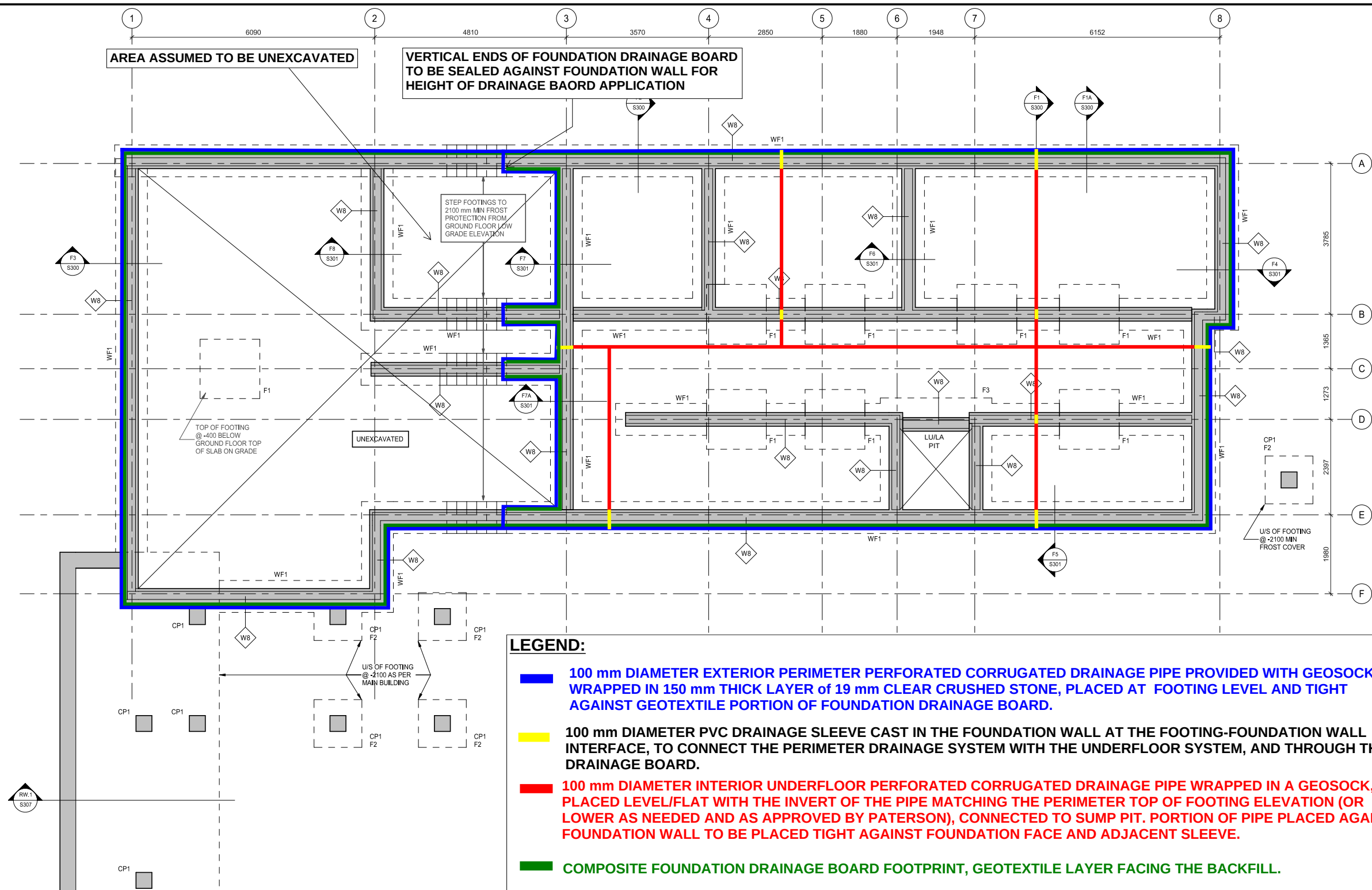
FIGURE 4 - PERIMETER AND UNDERFLOOR DRAINAGE SYSTEM
