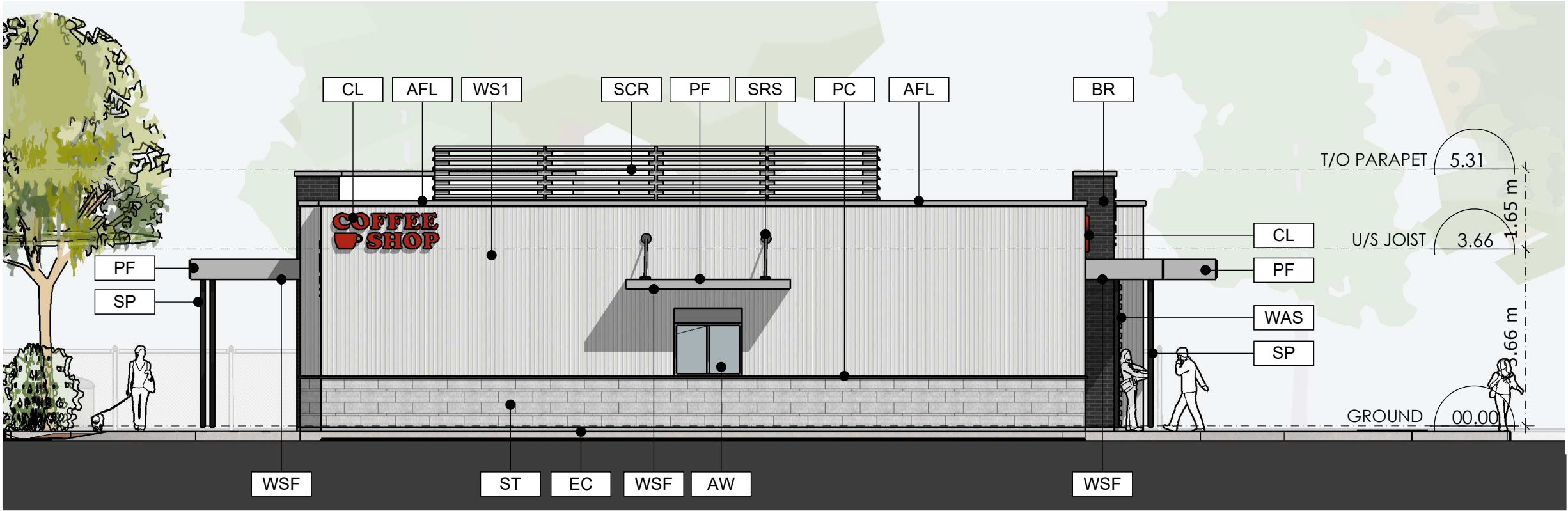
SOUTH ELEVATION
