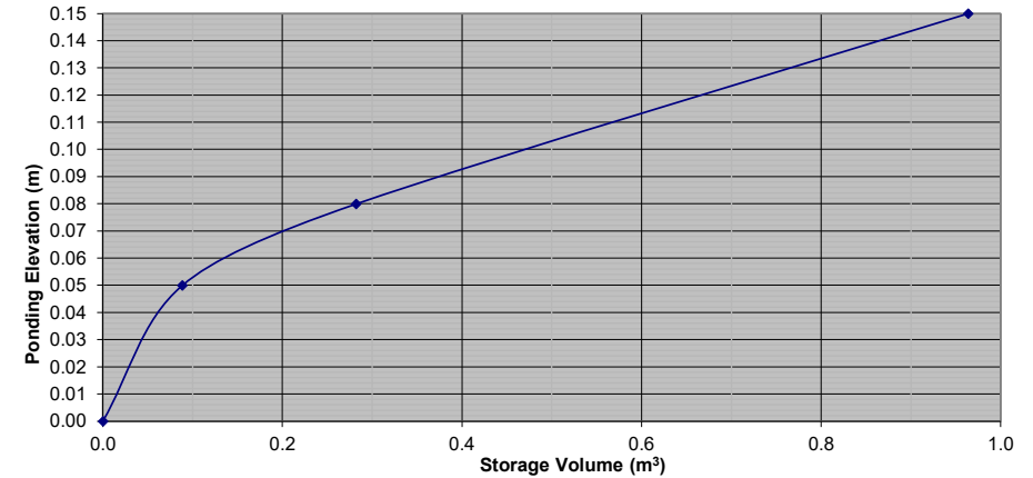
Stage Storage Curve: Area A-1.1 Controlled Roof Drain RD-16
