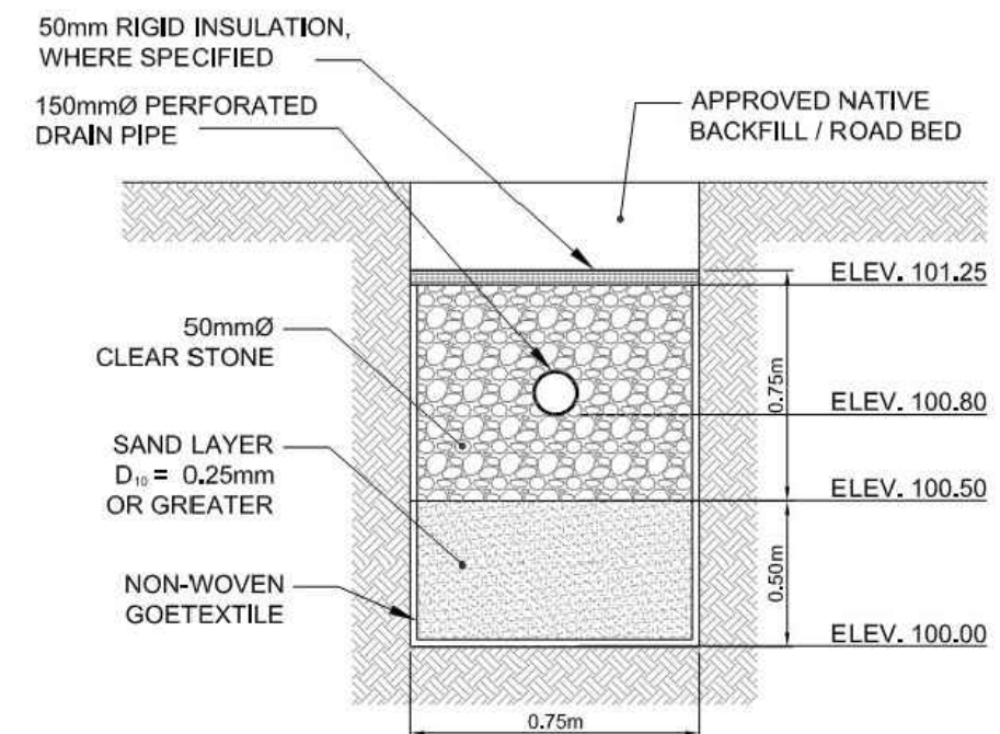
INFILTRATION TRENCH SECTION NOT TO SCALE
