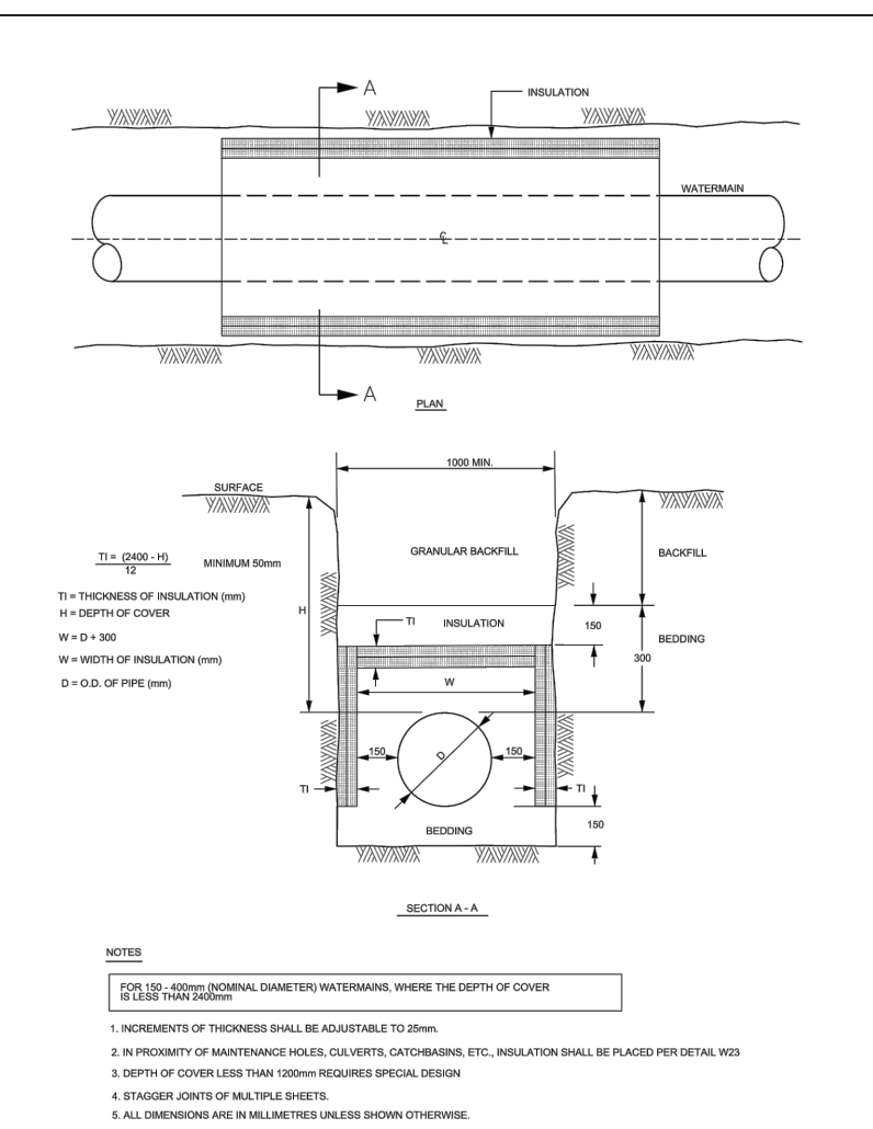
THERMAL INSULATION FOR WATERMAINS IN SHALLOW TRENCHES
