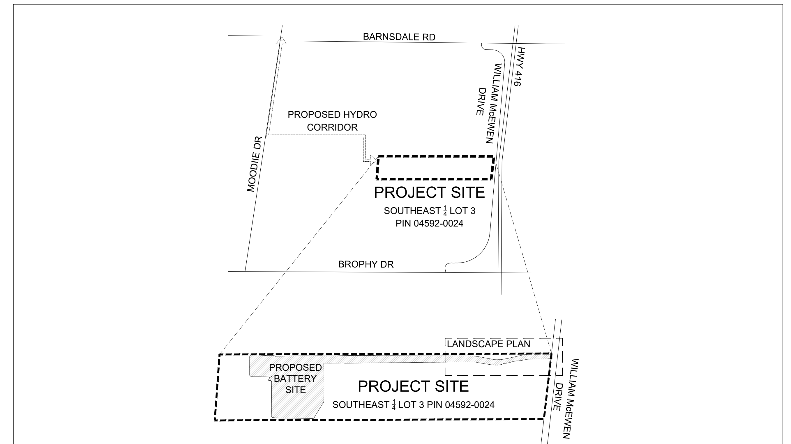
LOCATION PLAN
