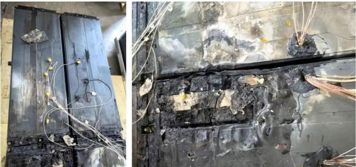
Figure 14 - Module Post-Test (Unit Level Test)
