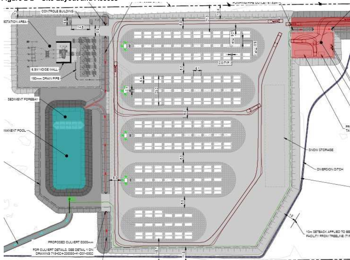
Figure 2-2 – Site Layout and Access
